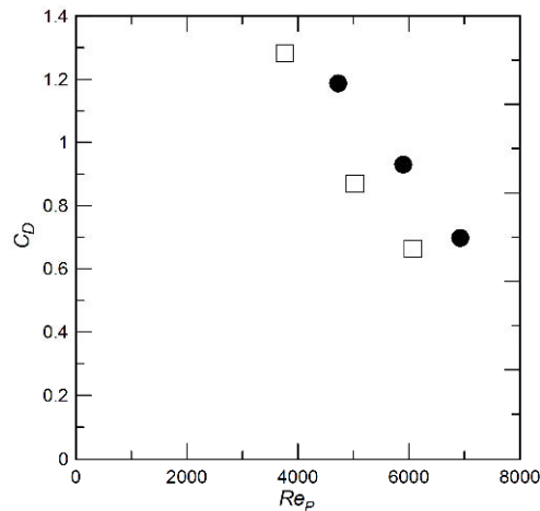
Fig. 7. Plant drag coefficient as a function of the plant Reynolds number Re_p = d_p U / \nu , for dense ( \square ) and sparse ( \bullet ) configurations.
