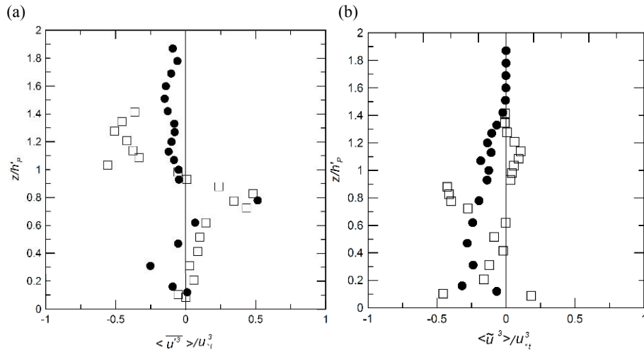
Fig. 14. Streamwise velocity third-order moment profiles for dense ( \square ) and sparse ( \bullet ) configurations: (a) spatially averaged contribution \langle \bar{u}^3 \rangle / u_{s_f}^3 ; (b) form-induced contribution \langle \tilde{u}^3 \rangle / u_{s_f}^3 .
