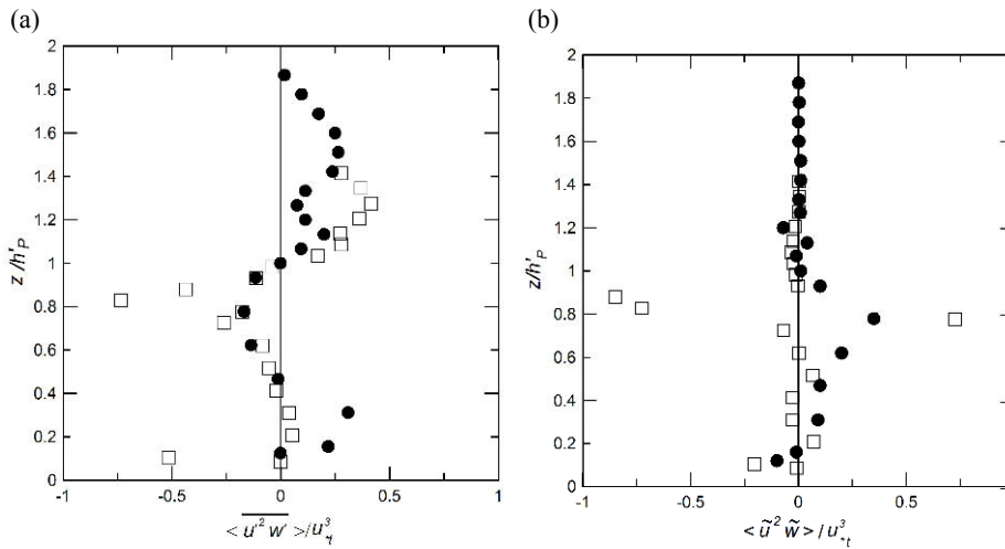
Fig. 15. Mixed third order velocity moment profiles for dense ( \square ) and sparse ( \bullet ) configurations: (a) spatially averaged contribution \langle \bar{u}^2 \bar{w}' \rangle / u_{s_f}^3 ; (b) form-induced contribution \langle \tilde{u}^2 \tilde{w}' \rangle / u_{s_f}^3 .
