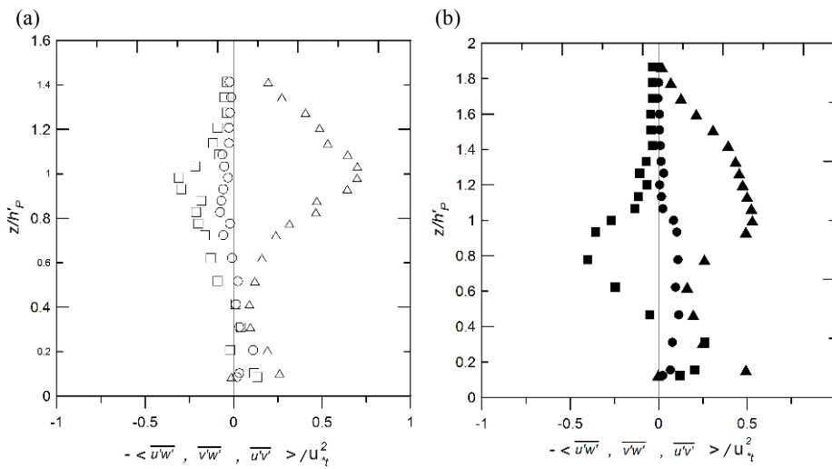
Fig. 9. Spatially averaged turbulent Reynolds profiles for dense and sparse configurations. (a) Dense configuration: \Delta \langle \overline{u'w'} \rangle / u_{*t}^2 , \square \langle \overline{u'v'} \rangle / u_{*t}^2 , \circ \langle \overline{v'w'} \rangle / u_{*t}^2 . (b) Sparse configuration: \blacktriangle \langle \overline{u'w'} \rangle / u_{*t}^2 , \blacksquare \langle \overline{u'v'} \rangle / u_{*t}^2 , \bullet \langle \overline{v'w'} \rangle / u_{*t}^2 .
