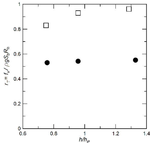
Fig. 6. Ratio between the plant drag per unit bed surface and streamwise momentum component for dense ( \square ) and sparse ( \bullet ) configurations.
