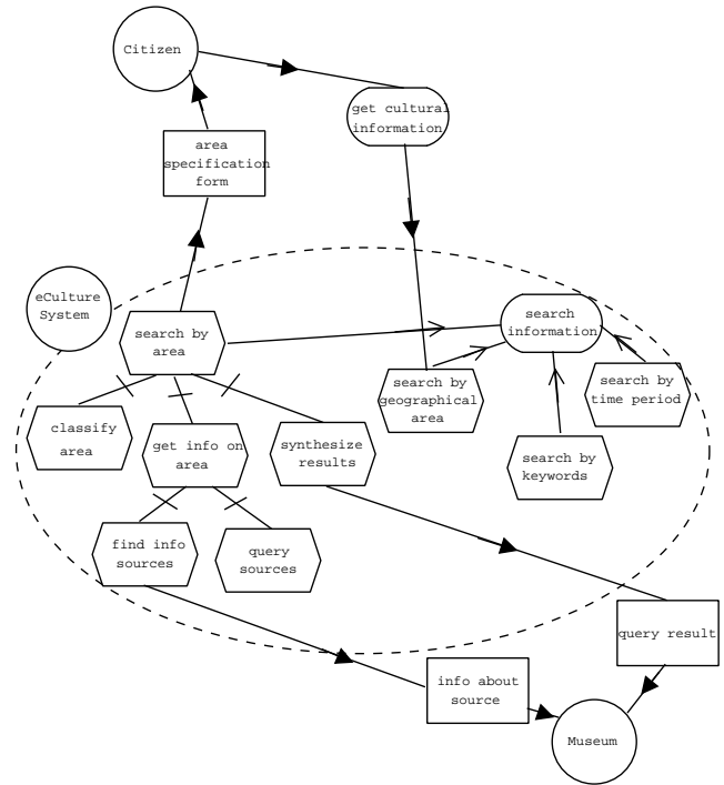
Figure 5: Rationale diagram for the goal get cultural information. Hexagonal shapes model tasks. Task decomposition links model task-subtask relationships. Goal-task links are a type of means-ends links.
