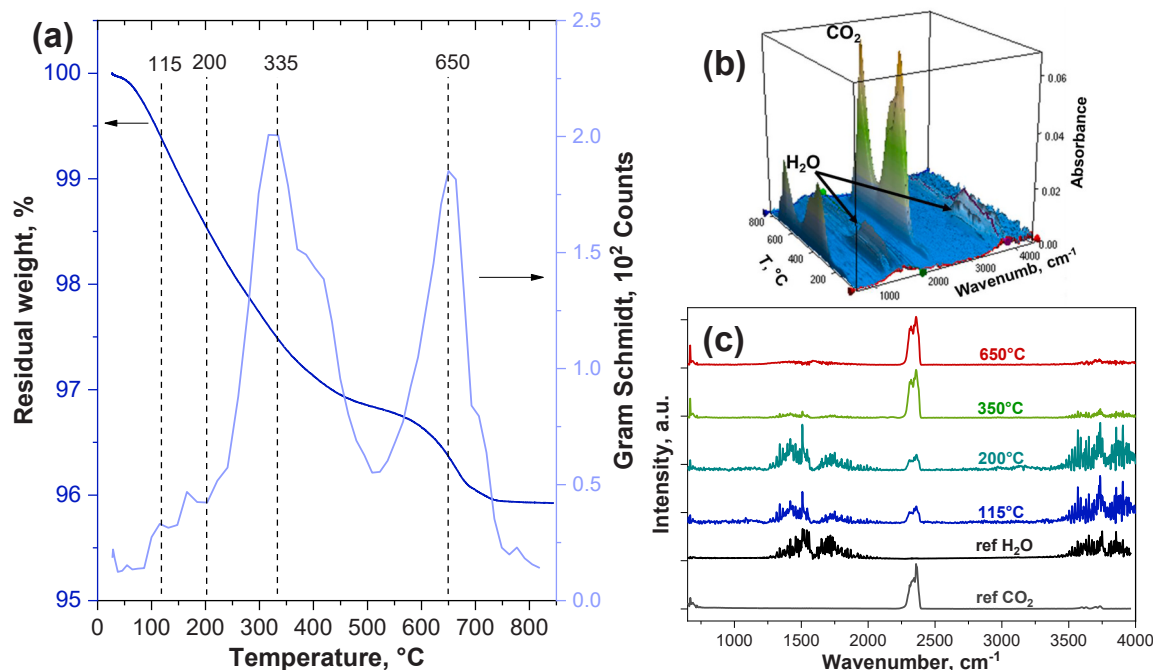
Fig. 4. (a) TGA and Gram-Schmidt curve as a function of temperature for 20 %_5M_200°C_500MPa sample; (b) FTIR absorbance evolution measured on the gas evolved from the sample in TGA, and (c) representative FTIR spectra at different temperatures. The reference spectra for carbon dioxide and water are also provided.
