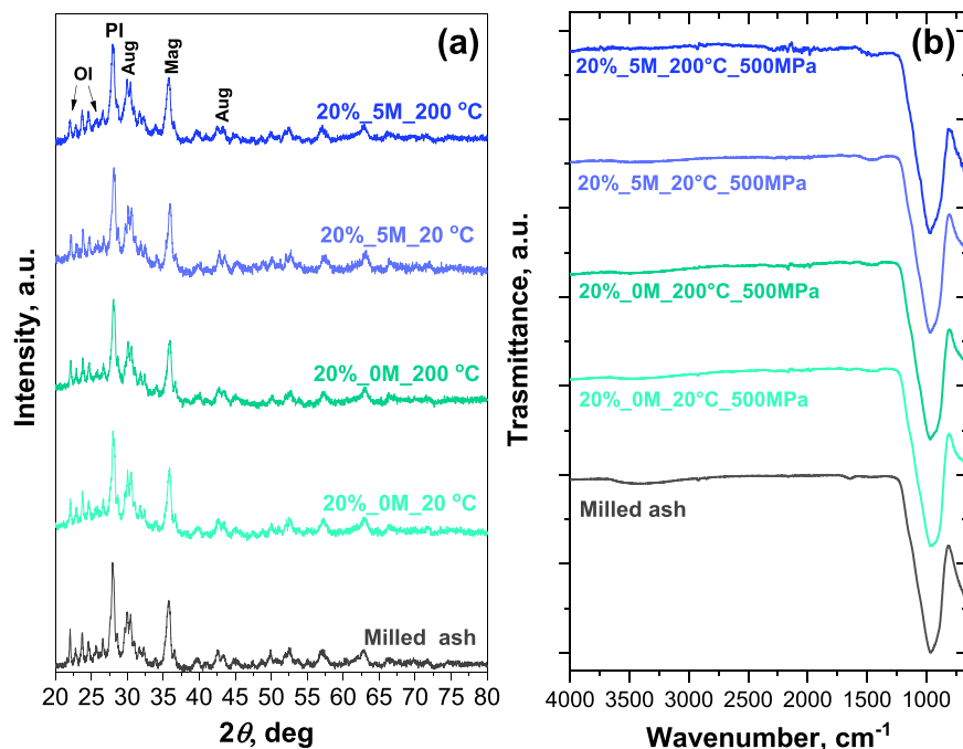
Fig. 3. (a) XRD patterns of the pristine ash and the cold sintered materials for different KOH solution molarity and processing temperature (pressure = 500 MPa). Pl = Ca-plagioclase (anortite), Aug = augite, Ol = olivine, Mag = Ti-magnetite (i.e., \text{Fe}^{2+}(\text{Fe}^{3+}, \text{Ti}^{3+})_2\text{O}_4 ). (b) FTIR spectra (ATR mode) of the pristine ash and the cold sintered materials for different KOH solution molarity and processing temperature (pressure = 500 MPa). The samples consolidated were dried overnight at 130°C.
