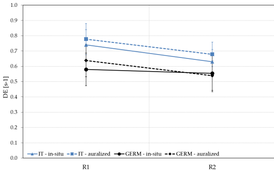
Fig. 9 – Comparison of listening efficiency values (DE) from real and auralized tests, for Italian (IT) and German (GERM) native speakers
