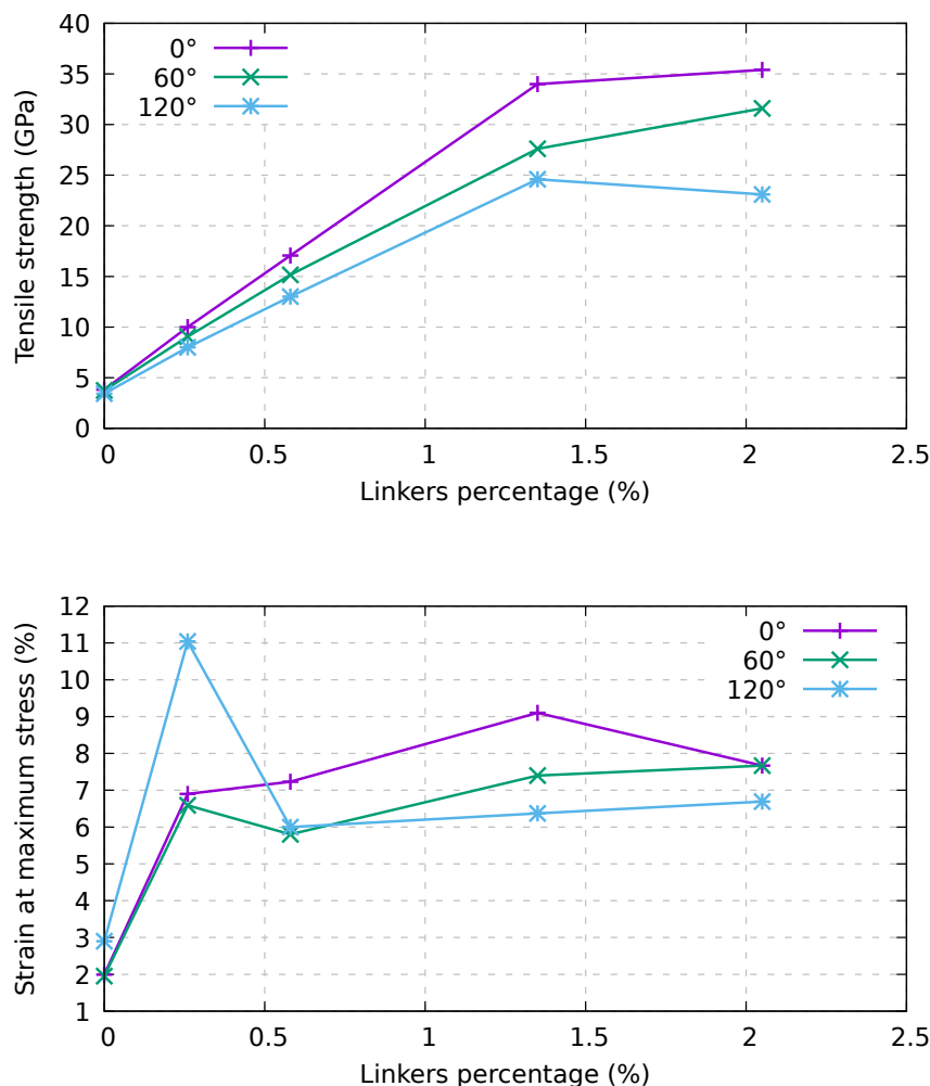
Figure 7. Dependence on twisting and percentage of linkers of the tensile strength ( top ) and strain at maximum stress ( bottom ) for an infinite bundle composed of (6, 6) CNTs with a periodic supercell of 20 nm in length. AIREBO-mod potential and a strain velocity of 1.0 Å/ps were used.
