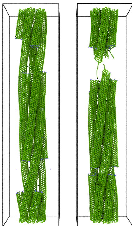
Figure 9. Snapshot at 15% strain of the 120° twisted bundle composed of 20 nm (6,6) CNTs for a percentage of linkers of 0.58% (left) and 1.53% (right). A different percentage of linkers corresponds to different failure mechanisms: the slipping of the nanotubes (left) and the fracture of the nanotubes (right), respectively.
