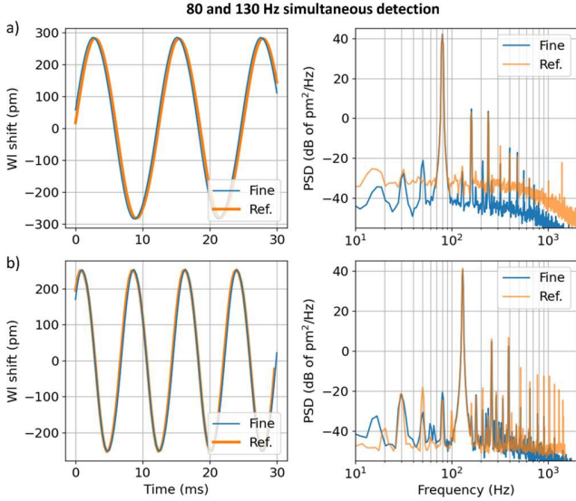
Fig. 5: Measured results using the fine interferometer applying two simultaneous signals at 80 Hz on channel at 1548 nm (a) and 130 Hz at 1540 nm (b). On the left we show the temporal signal, and on the right, the PSD of a 5s temporal trace.
