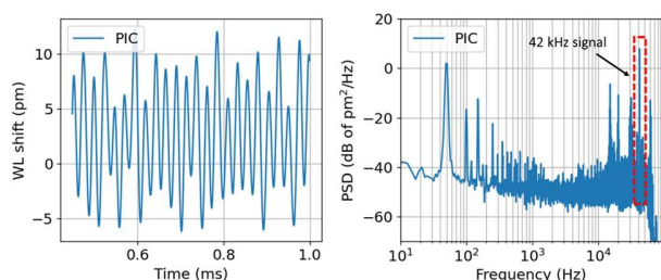
Fig. 10. Signal detection retrieved from the PIC when applying a 42 kHz signal at the FBG.
