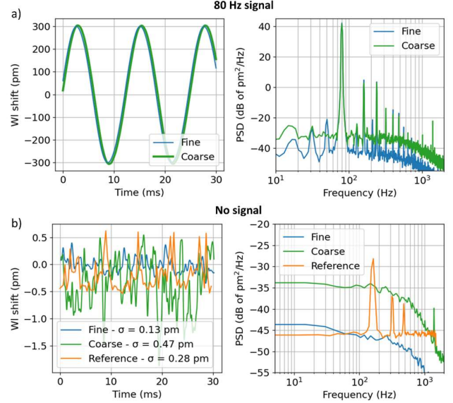
Fig. 6: Comparison between the coarse and the fine interferometer for the FBG at 1548 nm. (a) Applying signal at 80 Hz. (b) Noise measurement also compared with the reference interrogator
