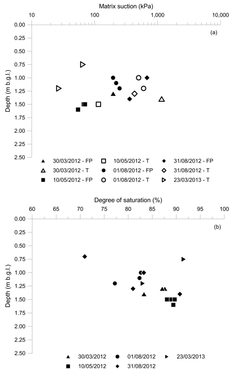
Figure 5. Water retention data of the Paola Doce fissured clay sampled at different depths and during different periods of the year: (a) matrix suction, measured with the filter paper technique, FP, and high-capacity tensiometers, T; (b) degree of saturation.
