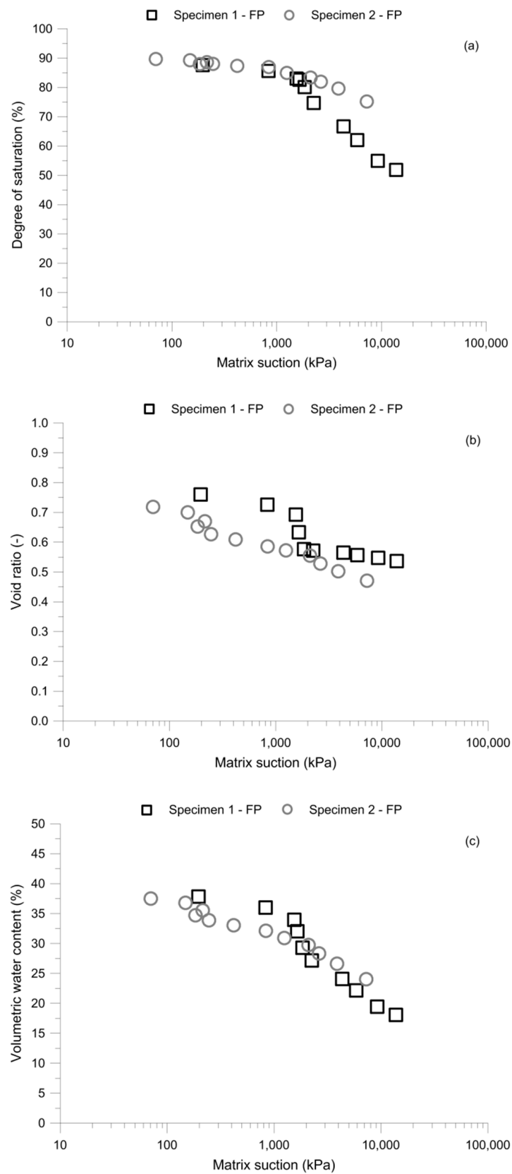
Figure 6. Representative water retention data of the Paola Doce fissured clay reported in terms of matrix suction (measured with the filter paper technique, FP) against: (a) degree of saturation; (b) void ratio; (c) volumetric water content.
