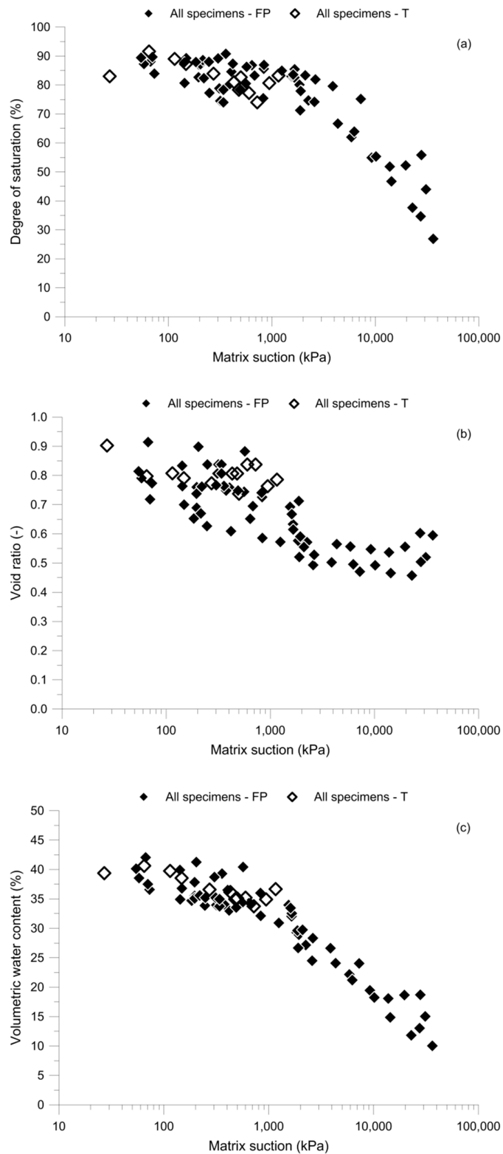
Figure 9. Water retention data of all the specimens (tested with both the filter paper technique, FP, and high-capacity tensiometers, T) reported in terms of matrix suction against: (a) degree of saturation; (b) void ratio; (c) volumetric water content.
