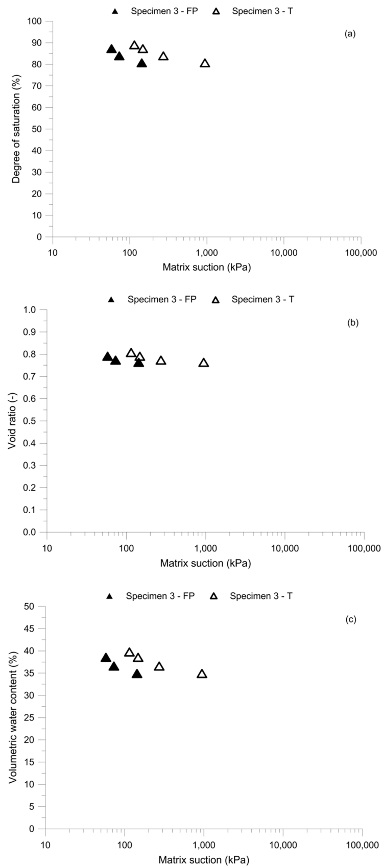
Figure 7. Water retention data of a specimen (tested with both the filter paper technique, FP, and high-capacity tensiometers, T) reported in terms of matrix suction against: (a) degree of saturation; (b) void ratio; (c) volumetric water content.
