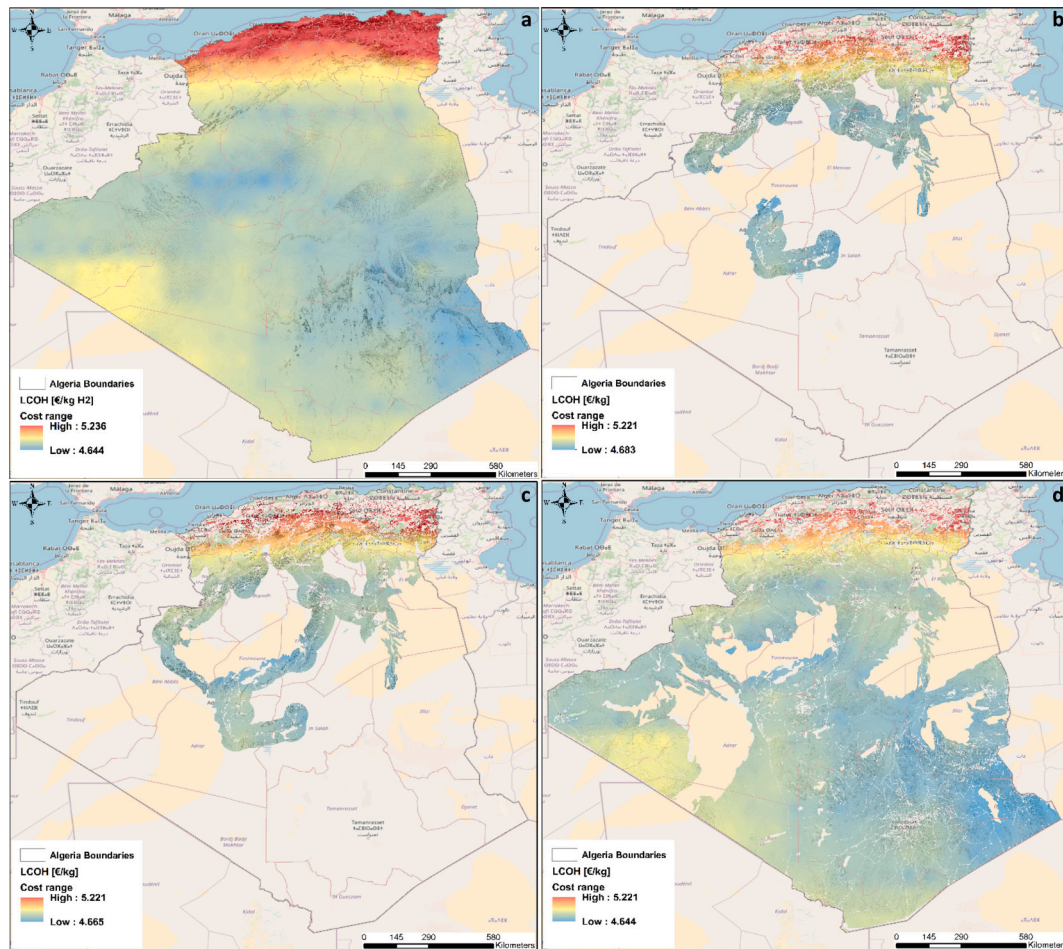
Fig. 9. Spatial distribution of the levelized cost of hydrogen (LCOH) from tilted PV-driven electrolysis across Algeria under grid-availability scenarios (a) baseline (unconstrained) LCOH, (b) LCOH in on-grid eligible areas, (c) LCOH along the on-grid North-South (N-S) interconnection corridor, and (d) LCOH in the off-grid eligible scenario. Units (€/kg H 2 ).
