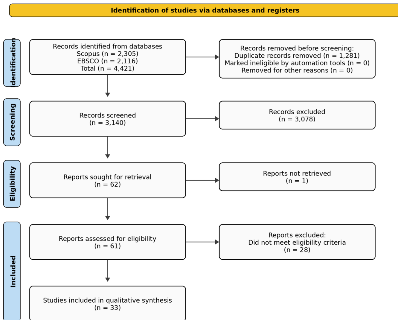
FIGURE 1 | PRISMA diagram.
