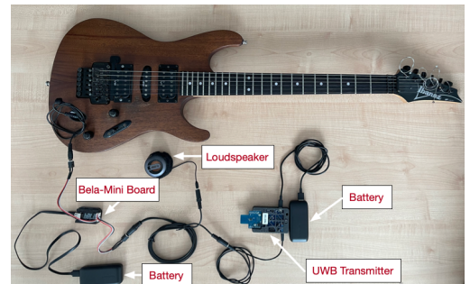
(b) Smart electric guitar (Prototype 2 and 4).
