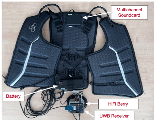
(b) Musical haptic vest (Prototype 3 and 4).
