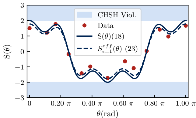
FIG. 7: S -parameters (experimental data and theoretical curves) in the incoherent regime. \eta = 0.89 \pm 0.01 and \epsilon = 1 were used in the calculation of the S_{\epsilon=1}^{eff} -parameter by (23). Error bars are within the dot size.
