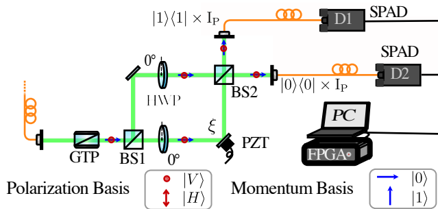
FIG. 9: Setup for the autocorrelation measurements
