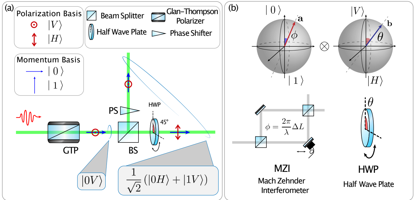
FIG. 2: (a) Setup for the generation of single-particle entangled states. (b) Momentum and polarization bases in the Bloch sphere and the optical elements constituting the preparation stage of Fig. 1.
