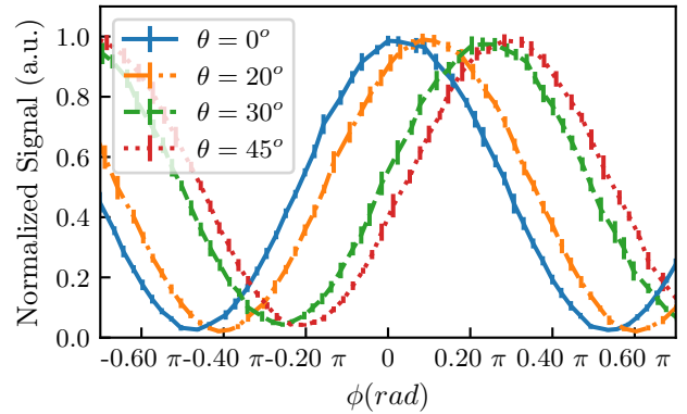
FIG. 6: Signal acquired by one single SPAD ( N_{OH}^{(a,b)} ) as a function of \phi for different polarization angles \theta in the coherent case. Counts are normalized to the maximum count in the set.
