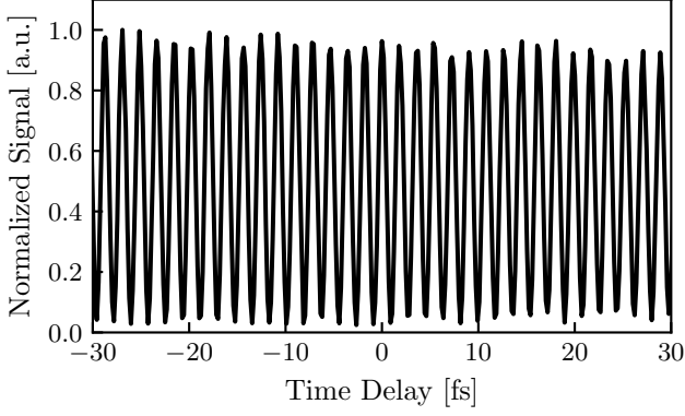
FIG. 11: Autocorrelation of the filtered LED.
