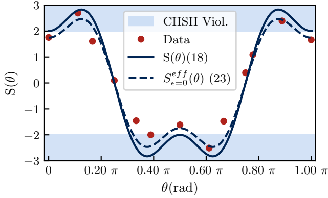
FIG. 4: Bell inequality measurement for a filtered (1nm bandwidth) LED and for the setup aligned within the coherent regime. Data points are experimental results while lines are theoretical curves (full line ideal S -parameter (18), dashed line S^{eff} -parameter (23) with \epsilon = 0 and \eta = 0.87 \pm 0.02 ). Error bars are within the dot size.
