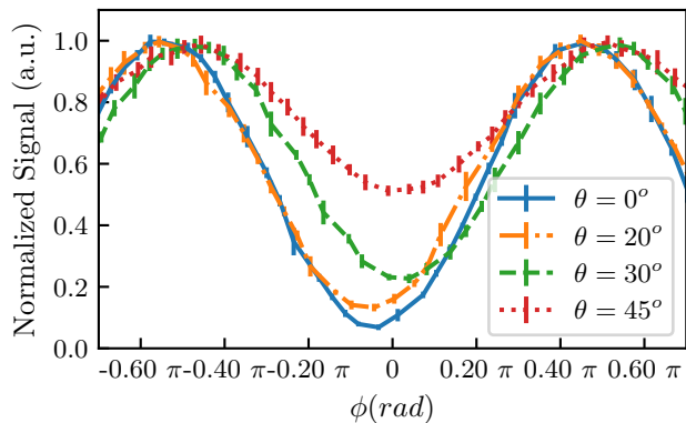
FIG. 8: N_{OH}^{(\phi,\theta)} as a function of \phi for different \theta for the incoherent case.
