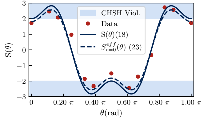
FIG. 5: Bell inequality measurements for a 1 nm filtered halogen lamp. Data points are experimental results while lines are theoretical curves (full line ideal S -parameter (18), dashed line S^{eff} -parameter (23) with \epsilon = 0 and \eta = 0.91 \pm 0.01 ). Error bars are within the dot size.
