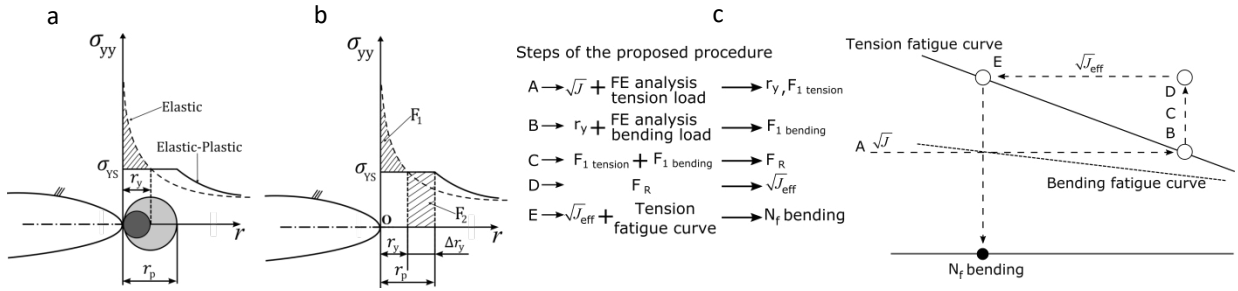
Fig. 3. Qualitative representation of the first-order r_y and second-order r_p plastic zone size (a), and (b) load redistribution and force equilibrium; (c) simplified diagram of the proposed procedure for the evaluation of the number of cycles to failure of laser stake-welded T-joints under bending load.
