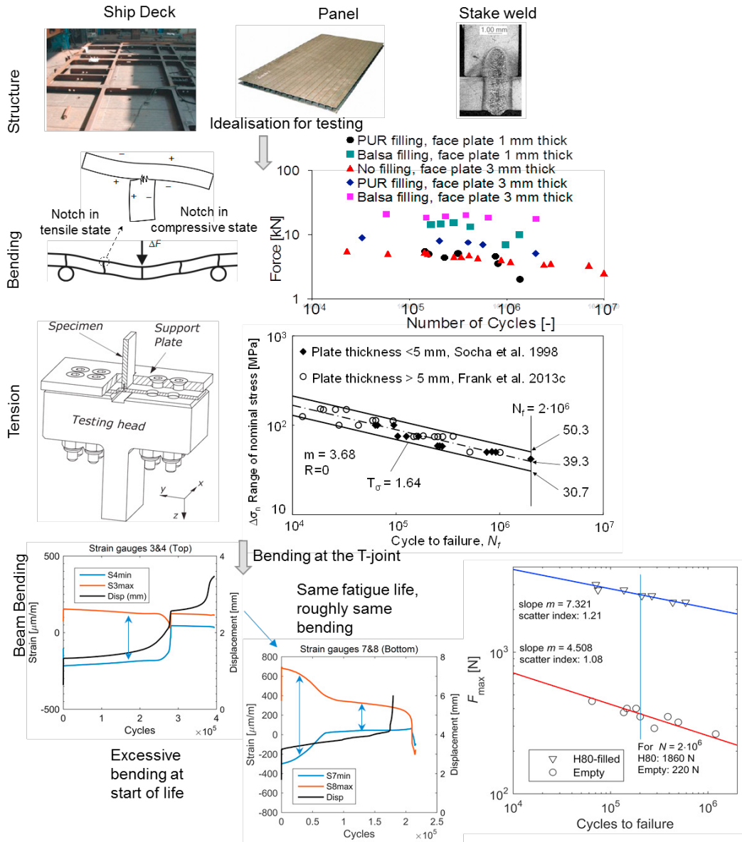
Fig. 1. Review on the fatigue strength test results on laser stake-welded T-joints by Socha et al. (1998), Sandwich Consortium (2002), Frank et al. (2013a), (2013c), Karttunen et al. (2017).
