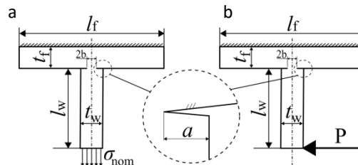
Fig. 4. Case study: laser stake-welded T-joint geometry under a) tension and b) bending load.
