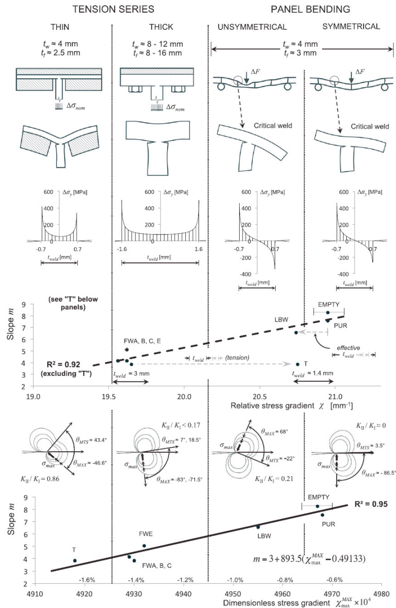
Fig. 2. The slope of fatigue resistance curve as a function of stress gradient, from Frank et al. (2013a).
