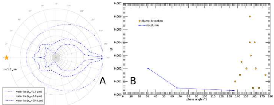
Fig. 20 Panel A: Variation of water ice scattering phase function with respect to grain size, evaluated at 1.2 μm wavelength through the Mie theory for lognormal distributions with effective radius of 0.5 μm (dotted line), 5 μm (dashed line), and 20 μm (dot-dashed line). The angular values on the grid represent the phase angle, hence the light source is at the left (star symbol). All curves are normalised to their maximum value, which is at 180° phase angle. Panel B: Enceladus plume reflectance level (~1.0–2.4 μm) resulting from a preliminary overview of a sample of Cassini/VIMS data as a function of solar phase angle (orange circles). Cases of non-detection are reported as upper limits in blue
