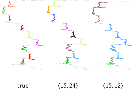
Fig. 15. Different stop properties, same unit quality. The figures represent the spatio-temporal view of a trajectory portion, showing the true stops and two sets of estimated stops determined with different SeqScan parameters. In each picture, points with different colors are units belonging to different stops; same colors across pictures do not denote an association of stops across them; gray points are move units.
