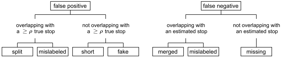
Fig. 7. A taxonomy of false detections.
