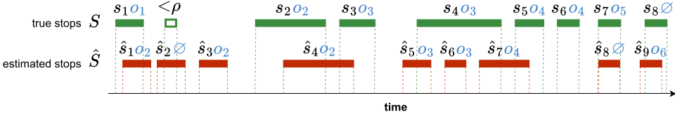
Fig. 6. Revisiting Figure 4 with semantic annotation of stops (POIs).
