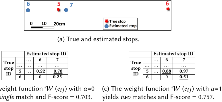
Fig. 19. The spatio-temporal weight \alpha may affect the F-score.
