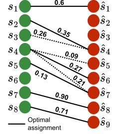
Fig. 5. Finding the matching set in Figure 4 based on temporal similarity.
