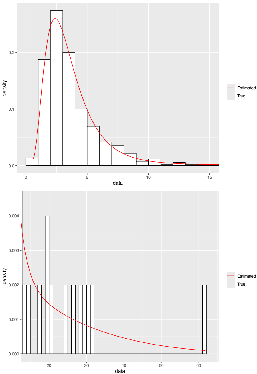
Fig. 3 Histogram of a simulated dataset from Case 1 ( n = 500 , \mu = 0 , \sigma = .5 , x_{min} = 5 and \alpha = 2 ), along with the true composite lognormal-Pareto density and the estimated lognormal-GPD static mixture density. Upper panel: distribution body ( x < 15 ). Lower panel: distribution tail ( x > 15 ). The bin width is the same in both panels.
