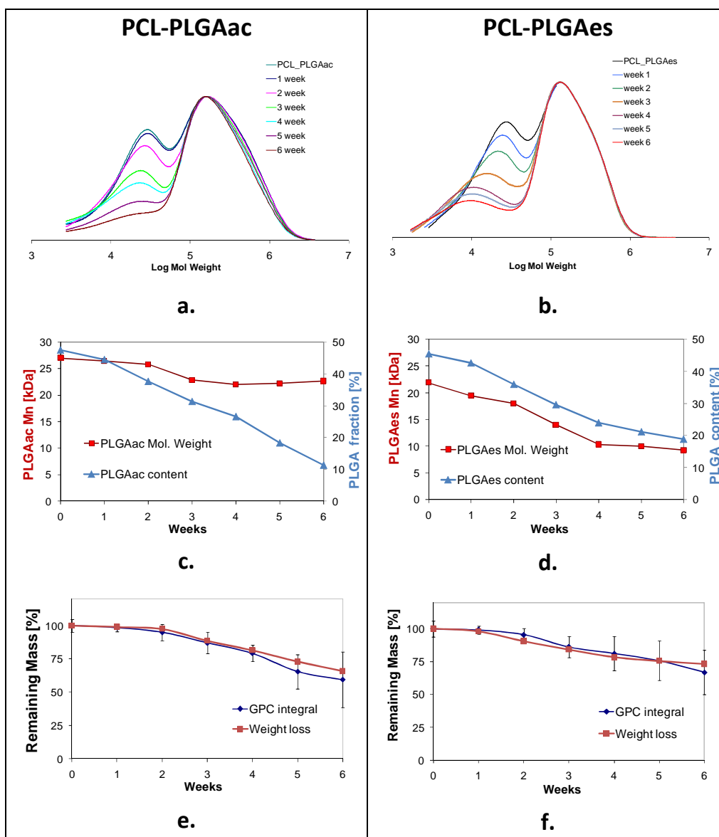
Figure 3-6. GPC analyses of PCL-PLGAac and PCL-PLGAes scaffolds as spun and after the hydrolytic degradation tests. (a - b) GPC curves of PCL-PLGAac and PCL-PLGAes; (c - d) Changes in number average molecular weight and remaining PLGA content determined by the deconvolution of the GPC curves; (e - f) Overall remaining mass percentage of the scaffolds determined by the gravimetric method and measurement of the total area under the GPC curves.
