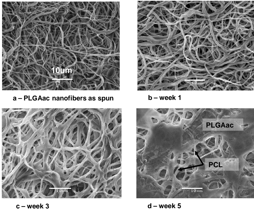
Figure 3-3. Representative SEM micrographs of the PCL-PLGAac nanofibrous scaffold with an internal compositional gradient. Images were taken from the PLGA side. (a) Morphology of PLGAac nanofibers as spun. (b-d) Changes in the nanofiber morphology after 1 week (b), 3 weeks (c), 5 weeks (d) of degradation in phosphate buffer solution at 37°C. The unchanged PCL nanofibers underneath the PLGAac layer were found after 5 weeks of degradation (d). Scale bar shows 10µm. Scale bar shows 10 µm.
