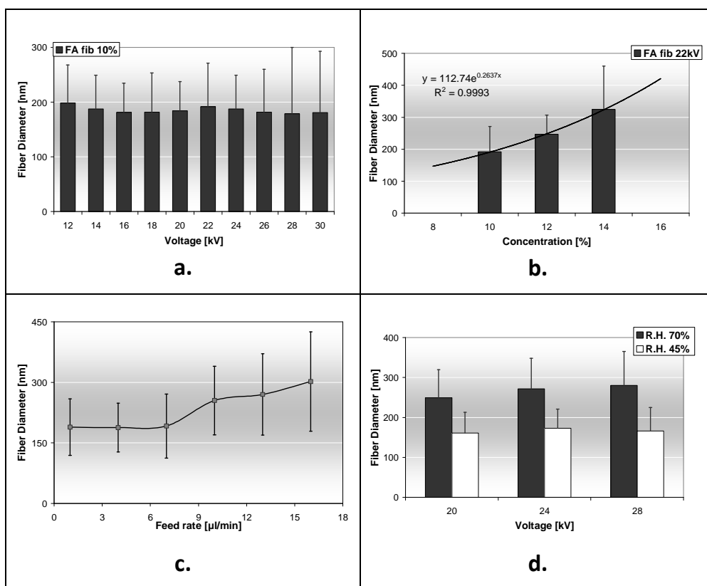
Figure 2-3. Effects of electrospinning process parameters on the mean fiber diameter of electrospun silk-fibroin: (a) applied voltage; (b) solution concentration; (c) feed rate; and (d) environmental relative humidity (R.H.). Effects of R.H were studied at different electrospinning voltages: 20 kV, 24 kV, and 28 kV.
