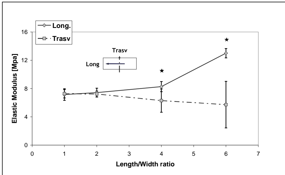
Figure 2-8. Effect of collector shape on the mechanical property of PCL electrospun material. Elastic modulus along the two principal directions of the electrospun nets is reported as function of the length/width ratio of the collector.
