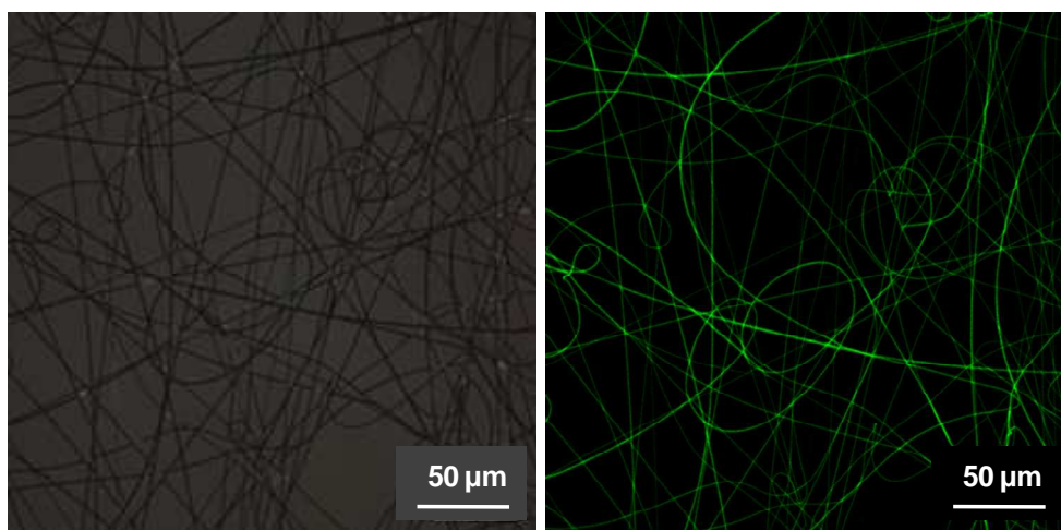
Figure 3-9. Optical and confocal images of PLGA nanofibers prepared by one-phase, solution electrospinning. Fluorecently-labeled, AlbF was dissolved directly in the polymeric solution and was homogeneously distributed along the nanofibers.
