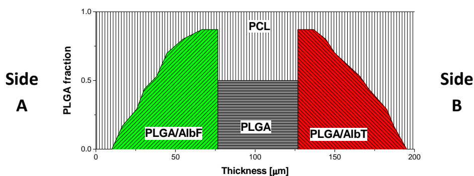
Figure 4-7. Modified PCL-PLGA scaffold with inverse gradient for dual molecule release from opposite sides of the scaffold and in vitro release profiles of AlbF and AlbT from the two surfaces of the scaffold. Schematic representation of a PCL-PLGA graded scaffold with two reversed gradients. The content of albumin-loaded PLGA nanofibers was 0 near the surfaces and maximum in the internal part of the scaffold. PLGA and PCL nanofibers were combined in the transition region between AlbF-loaded and AlbT-loaded PLGA nanofibers
