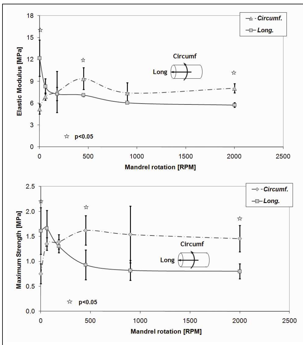
Figure 2-5. Elastic modulus and ultimate strength of silk-fibroin electrospun nets produced with a rotating collector. These properties in both longitudinal and circumferential directions change with the rotation speed. “☆” shows that the mechanical property of the sample in the longitudinal direction is significantly different from that in the circumferential direction ( p < 0.05 ).
