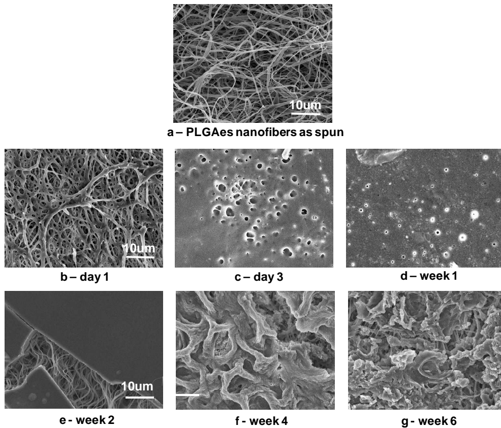
Figure 3-4. Representative SEM micrographs of the PCL-PLGAes nanofibrous scaffold with an internal compositional gradient. Images were taken from the PLGA side. (a). Morphology of PLGAes nanofibers as spun. (b-f) Changes in the PLGAes nanofiber morphology after 1 day (b), 3 days (c), 1 week (d), 2 weeks (e), 4 weeks (f) and 6 weeks (g) of degradation in phosphate buffer solution at 37°C. The unchanged PCL nanofibers underneath the PLGAes layer were found in all these images (b-d). Scale bar shows 10µm.
