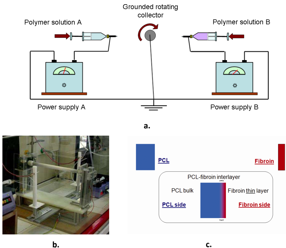
Figure 2-1. (a) Schematic illustration of the double electrospinning system; (b) Actual setup of the system; (c) Illustration of the PCL_fibroin multilayered material.
