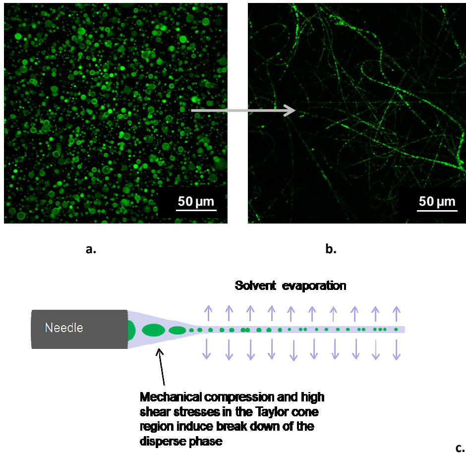
Figure 5-3. Confocal images of a W/O emulsion of AlbF in and the corresponding electrospun nanofibers. a.) W/O emulsion consisting a 2mg/ml water solution of ALbF dispersed in a 17% (wt) solution of PLGA in CL (water phase/organic phase ratio equal to 1/20); b.) AlbF distribution in AlbF-loaded PLGA nanofibers obtained by electrospinning of the emulsion; c.) Schematic illustration of the microdroplets breakdown in the region of the Taylor cone and the formation of fluorescent nanoclusters along the nanofibers during electrospinning
