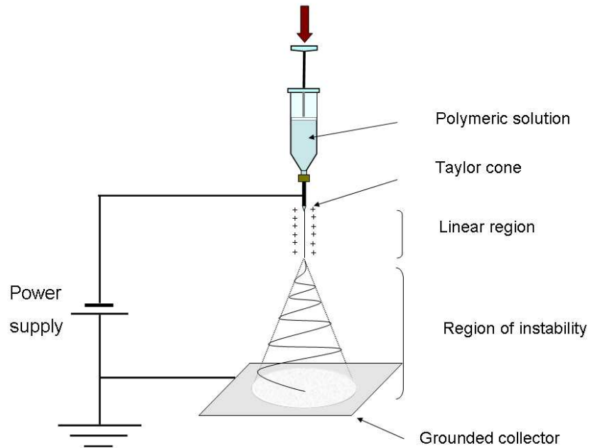
Figure 1-1. Schematization of the electrospinning process
