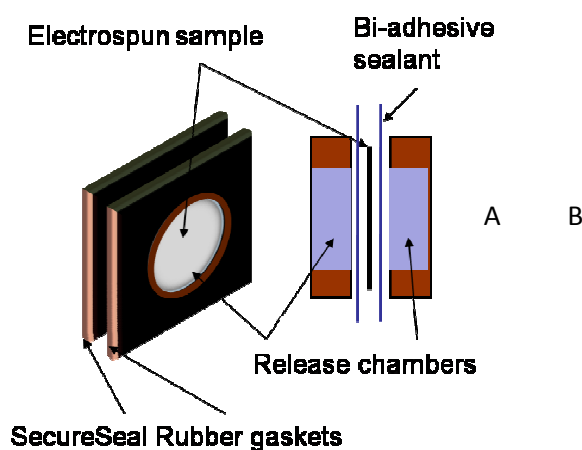
Figure 3-7. Schematic illustration of the custom-made diffusion chambers with independently sealed reservoirs facing the two surfaces of the electrospun samples.
