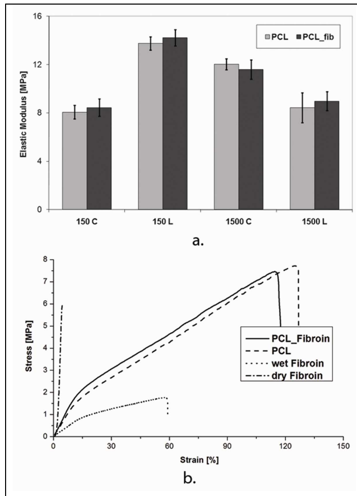
Figure 2-11. a) Elastic modulus of multilayered PCL-fibroin materials and pure PCL materials. The material fabrication used a cylindrical collector rotating at a low speed (150 rpm) and a high speed (1500 rpm). All the tests were performed on the circumferential direction “C” and the longitudinal direction “L” of the samples. No significant differences in elastic modulus were found ( p > 0.05 ). b) Representative stress-strain curves of hydrated fibroin, dry fibroin, PCL, and PCL-fibroin electrospun nets. The material fabrication used a cylindrical collector rotating at a high speed (1500 rpm). All the tests were performed on the circumferential direction of the tubular scaffolds.
