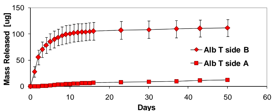
Figure 3-10. Cumulative release of AlbT from the two surfaces of PCL-PLGAac composite scaffolds. The scaffolds were prepared following the compositional pattern presented in Table 3-1. AlbT was encapsulated in PLGAac and it was released mainly from the PLGAac-rich side. “Side A” refers to the PCL-rich side, whereas “Side B” refers to the AlbT-loaded PLGAac side.
