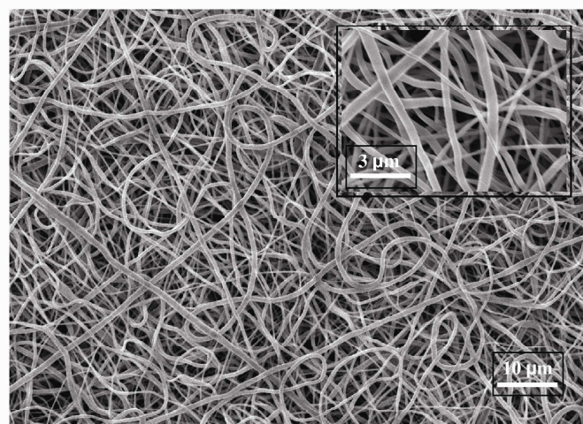
Figure 2-2. SEM imaging graphs of silk-fibroin nanofibers (a) and PCL nanofibers (b) (scale bar = 10 μm). At a higher magnification, details of fiber morphology are shown (scale bar = 3 μm). The electrospinning processes were conducted on a flat aluminium collector with RH = 70% and optimized electrospinning parameters listed in Table 1.
