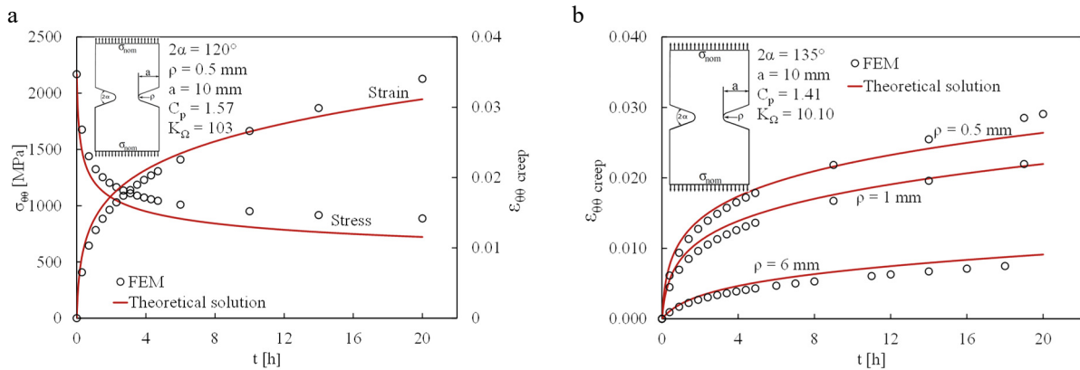
Fig. 2. Comparison between theoretical and FEM evolution of stress and strain as a function of time for V-notch geometry: (a) \rho = 0.5 mm, 2\alpha = 120^\circ ; (b) 2\alpha = 135^\circ and \rho = 0.5, 1, 6 mm.
