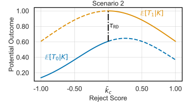
Figure 3: Scenario 2 assumptions: thick (dashed) lines are observed (unobserved) values. We can estimate \tau_{RD} at the cutoff value.
