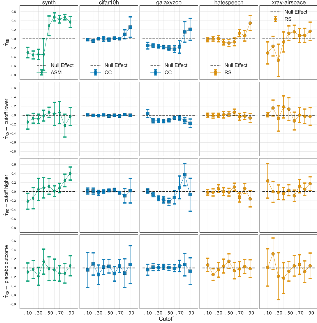
Figure 5: Estimated \hat{\tau}_{RD} for the best baselines over the five datasets. The first row provides the estimates of \hat{\tau}_{RD} . The second row provides the estimates for the lower cutoff placebo test. The third row provides the estimates for the higher cutoff placebo test. The fourth row provides the estimates for the placebo outcome test.
