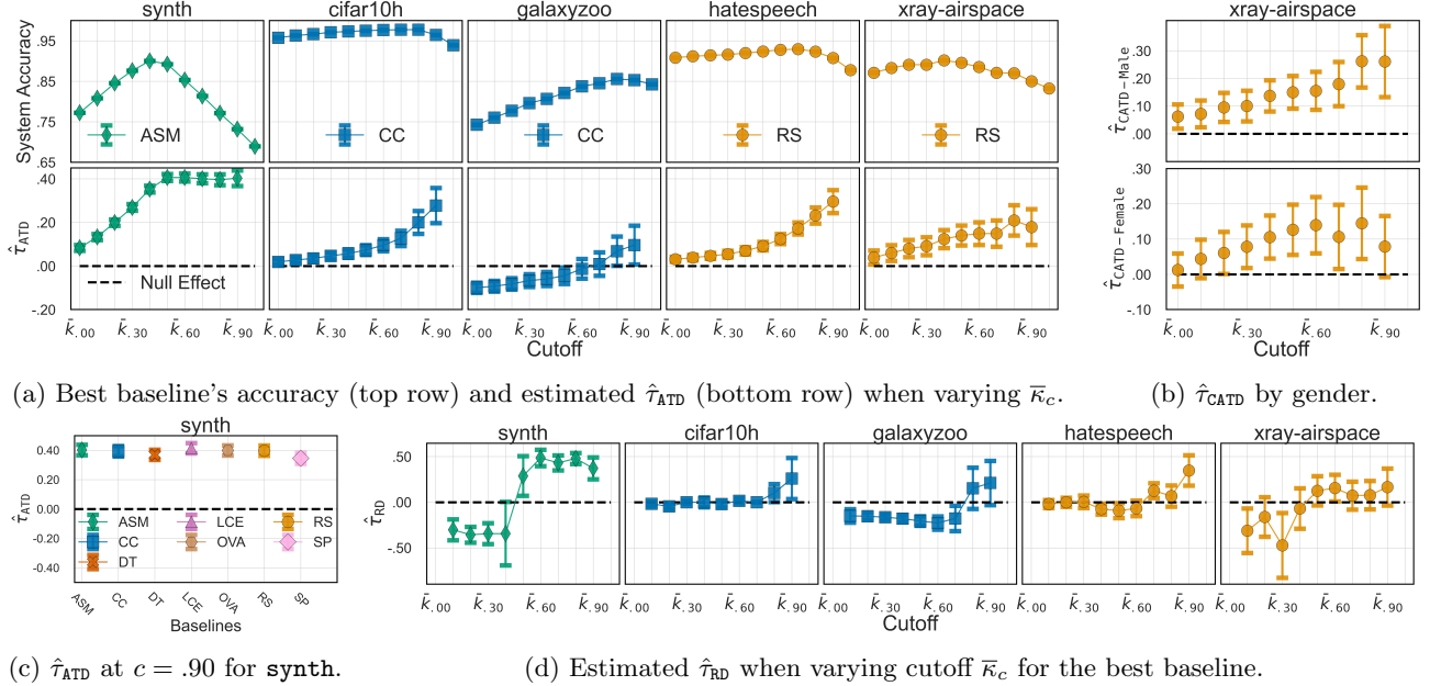
Figure 4: Experimental results: Figure 4a reports system accuracy and \hat{\tau}_{ATD} (Scenario 1); Figure 4b reports estimated \hat{\tau}_{CATD} when conditioning on the gender of the patient on the xray-airspace dataset; Figure 4c compares \hat{\tau}_{ATD} over multiple baselines on synth ; Figure 4d reports \hat{\tau}_{RD} (Scenario 2).
