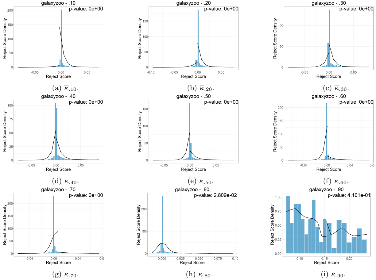
Figure 8: galaxyzoo estimated reject scores densities at the left and right of cutoff \bar{\kappa}_c for the best baseline CC. All the plots are zoomed around the cutoff values.
