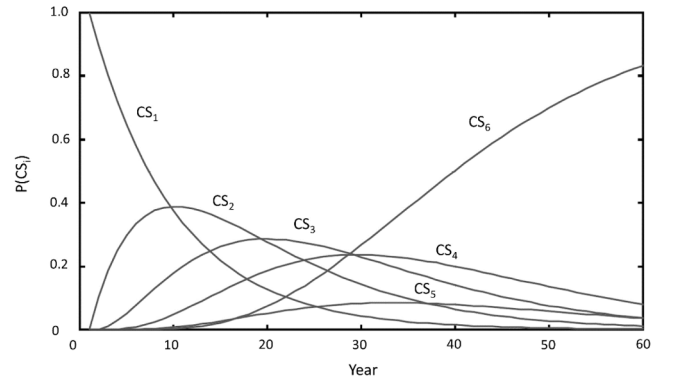
Fig. 12. Probability of being in a condition state vs time. Adapted from [151].
