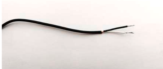
Fig. 13. Exposed end of the contact microphone wire after both of the conductors have been soldered, and the outer conductor has been insulated with heat shrink tubing.
