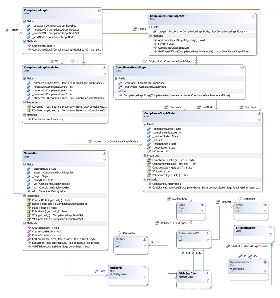
Figure 9: Simulation Class Diagram
