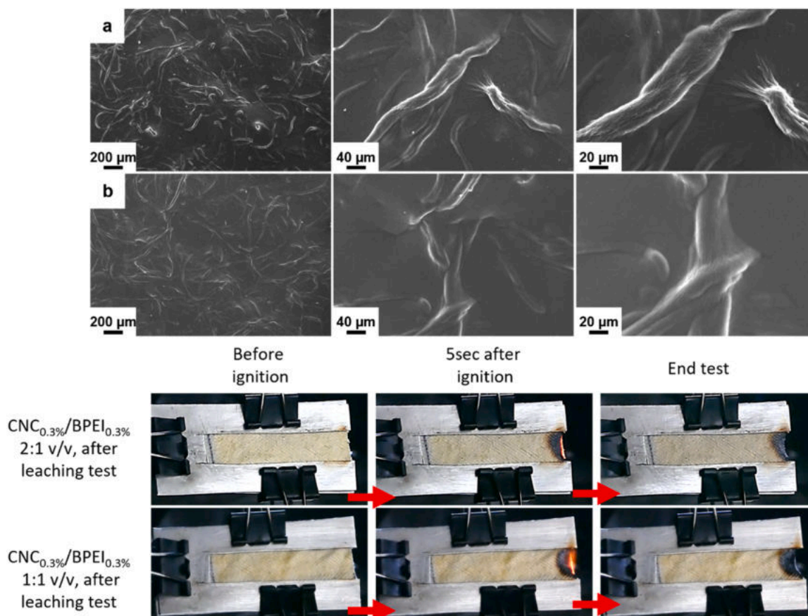
Fig. 6. Durability study: morphology by SEM and flammability results of \text{CNC}_{0.3\%}/\text{BPEI}_{0.3\%} 2:1 v/v and \text{CNC}_{0.3\%}/\text{BPEI}_{0.3\%} 1:1 v/v.
