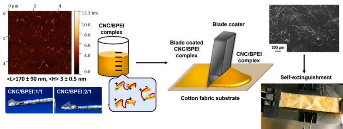
Fig. 1. Scheme of the work: AFM topography of obtained CNC and CNC/BPEI preparation procedure and deposition with flammability test.
