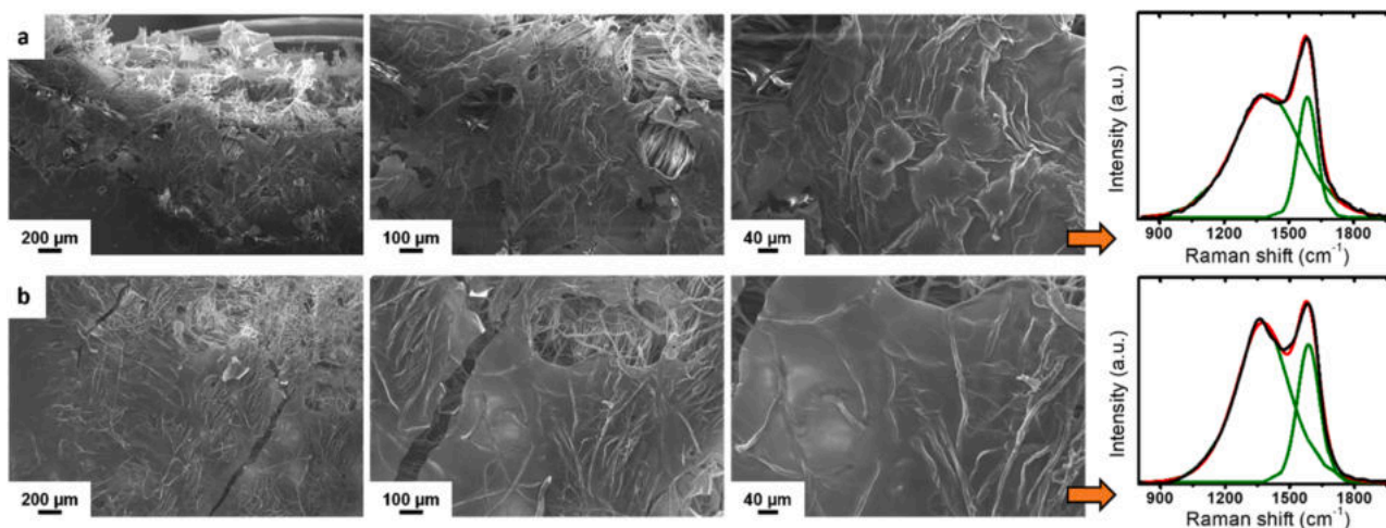
Fig. 7. SEM micrographs and Raman spectra characterization of post-combustion residues collected from \text{CNC}_{0.3\%}/\text{BPEI}_{0.3\%} 2:1 v/v (a) and \text{CNC}_{0.3\%}/\text{BPEI}_{0.3\%} 1:1 v/v after leaching test (b).
