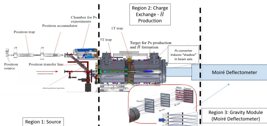
Figure 3: The AEgIS apparatus separated into source, \bar{H} production, and moiré deflectometer regions.
