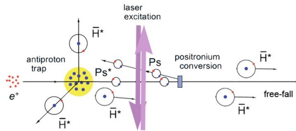
Figure 1: This schematic illustrates how \bar{H} is produced within the magnetic traps of AEgIS, when a positron-positronium converter is used. [20][21]
