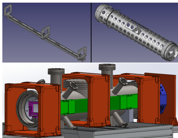
Figure 4: 3D drawing for the inner most section of the tube, the linear guide holding the moiré gratings (top left). The linear guide fixed to the rotating tube (top right). 3D drawing of the gravity module to be attached to AEgIS (bottom). Grating holders (pink), box scintillator detectors (red), JPET scintillator detector (green), and OPHANIM camera system (blue) is shown.
