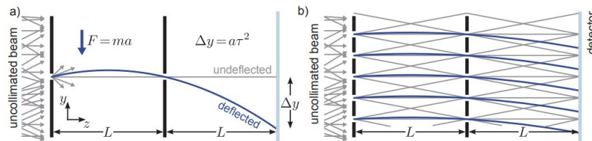
Figure 2: The difference in trajectories of a massive particle (blue) and an undeflected particle (gray) from a single slit grating are shown (a). Several trajectories from multiple slit grating are shown (b).[27]
