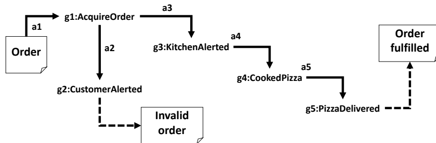
Figure 1: Agent-based workflow for the pizza delivery process.
