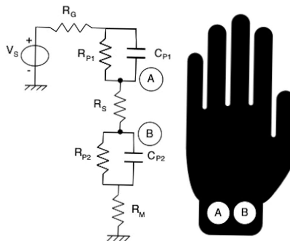
Fig. 1 Schema of galvanic skin resistance measurement
