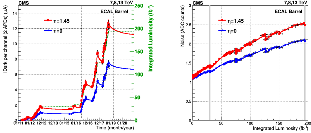
Figure 3. The APD dark current (IDark) evolution versus time in EB (left), in red for the channels at |\eta| = 1.45 and in blue for the channels at \eta = 0 , with the continuous lines representing the prediction of the model. The delivered integrated luminosity since the beginning of Run 1 is also shown in green. The scale of the integrated luminosity axis is chosen such that it tends to overlap with the dark current at |\eta| = 1.45 , in order to emphasize visually the strong correlation between dark current and integrated luminosity. The vertical bars on the points represent the uncertainty in the dark current measurement. On the right, the APD noise estimated from the dark current (continuous line) is compared with the direct noise measurement (data points) for the two \eta regions. The vertical grey lines in the right plot indicate the region corresponding to Run 2. The horizontal bars on the points represent the uncertainty on the luminosity.
