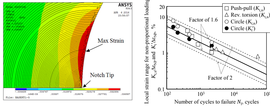
Figure 3. Contour plot of strain (a) and application of K' in the original Itoh-Sakane Model (b)
