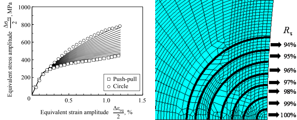
Figure 1. Curves between push-pull and circle (a) and areas to which a curve was assigned following R_t (shear stress percentage value) (b)
