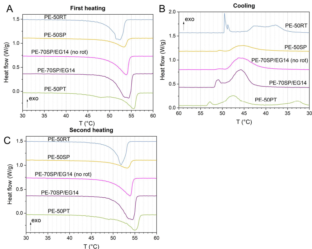
Figure 6. DSC thermograms of the HDPE-based samples at 1 °C/min. (A) First heating; (B) Cooling; (C) Second heating.
