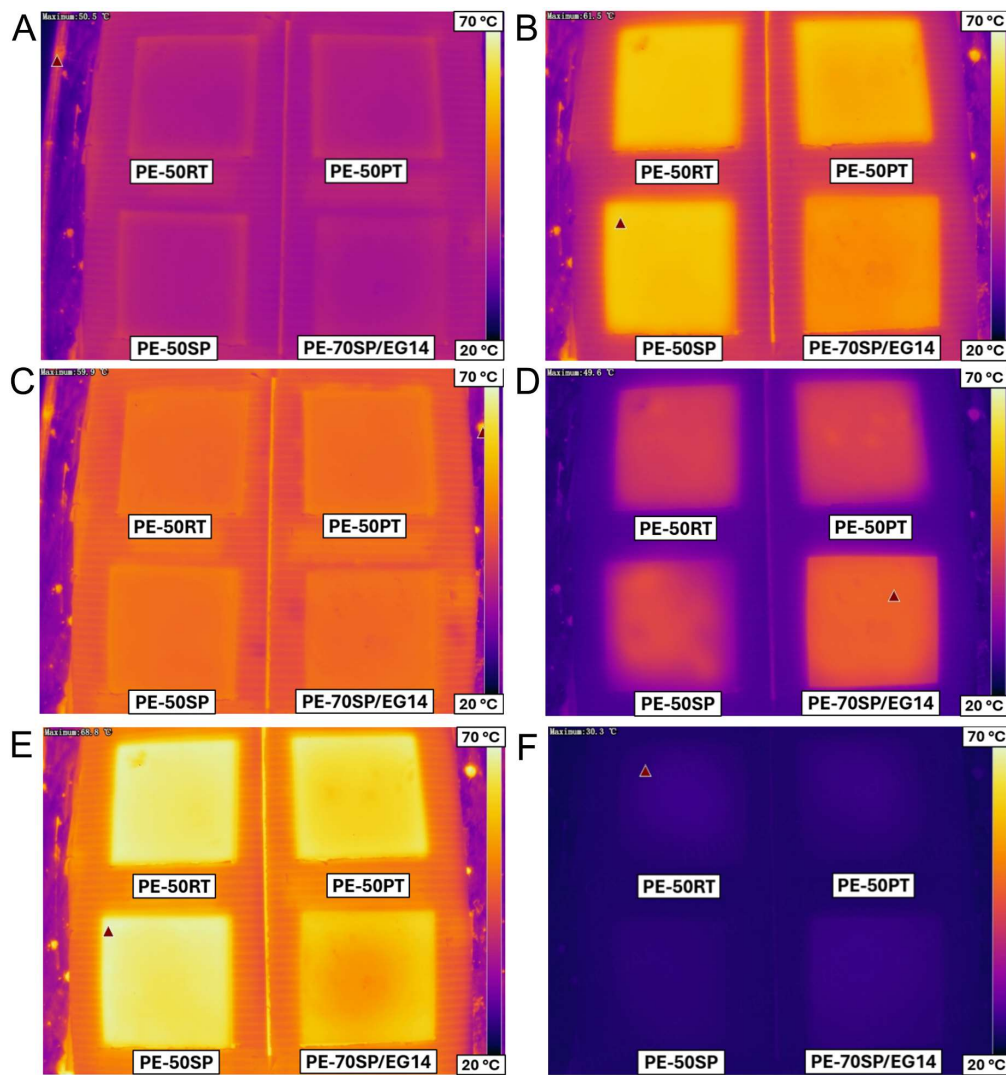
Figure 14. IR thermography images during heating (left) and cooling (right) of the sheets 120 \times 120 \times 3 mm 3 shown in Figure 2 after: 2 min (A and B), 15 min (C and D) and 45 min (E and F).
