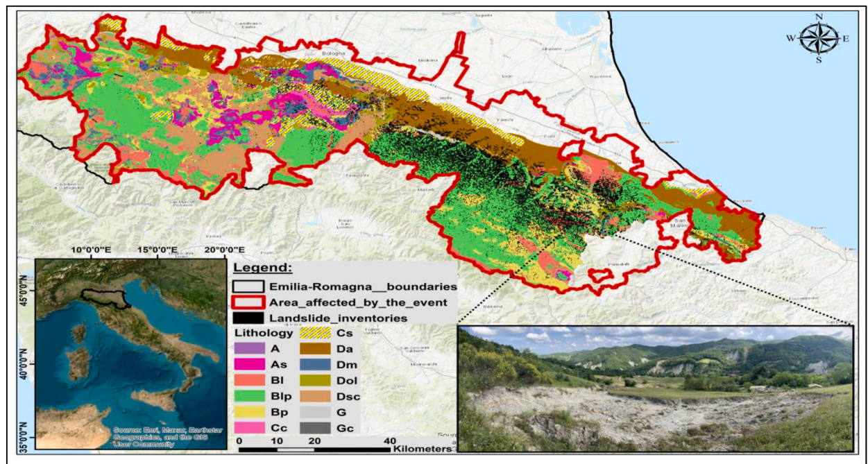
Fig. 1. Location of the study area. The area most affected by the event is displayed over the lithology classes. The left inset shows the location of Emilia–Romagna within Italy, while the lower right inset presents a representative field photo of the study area.
