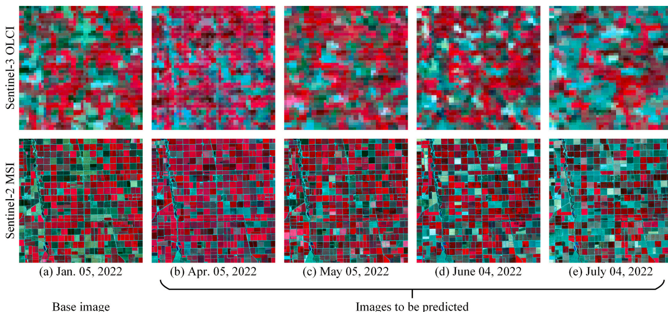
Fig. 5. Experimental data of the IC site. (a) Sentinel-2 MSI and Sentinel-3 OLCI image pair acquired on Jan. 05, 2022, (b)-(e) four Sentinel-2 MSI and Sentinel-3 OLCI image pairs acquired on Apr. 05, 2022, May 05, 2022, June 04, 2022, and July 04, 2022, respectively. All images use NIR-red-green as RGB false colour composition. (For interpretation of the references to colour in this figure legend, the reader is referred to the web version of this article.)
