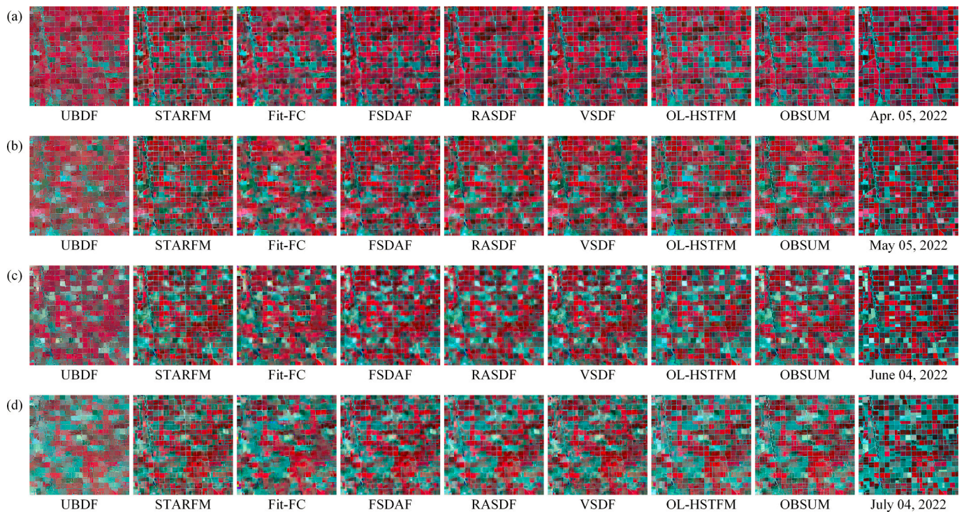
Fig. 12. Results of different spatiotemporal fusion methods on four prediction dates and the reference images at the IC site. All images use NIR-red-green as RGB false colour composition. (For interpretation of the references to colour in this figure legend, the reader is referred to the web version of this article.)
