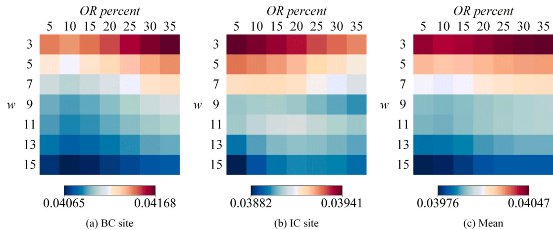
Fig. 6. RMSE of the images fused by OBSUM with different combinations of w and OR percent. (a) BC site when predicting the fine image on July 23, 2022, (b) IC site when predicting the fine image on June 04, 2022, and (c) mean value of two sites.
