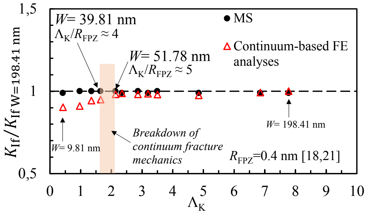
Figure 5. Normalized stress intensity factors at failure obtained from FE and MS analyses plotted against the length of the singular stress field, \Lambda_K , evaluated based on the stress fields from continuum-based FE analyses; \Lambda_K is defined as the distance from the crack tip at which the stress deviates more than 5% from expected 1/r^{0.5} singularity; picture includes values of the fracture process zone R_{FPZ} taken from the literature; from right to left, the points correspond to decreasing specimens width W , starting from W=198.41 \text{ nm} (far-right points) to W=9.81 \text{ nm} (far-left points); Table 1 reports numerical values.
