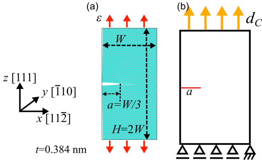
Figure 1. Schematics (a) of the cracked samples and simulation box employed in the molecular statistics analyses (visualized through OVITO [52] ), orientation, and (b) constraints configuration of FE model with critical displacement; t is the thickness of the simulation cell; the crack is slightly open to facilitate visualization.
