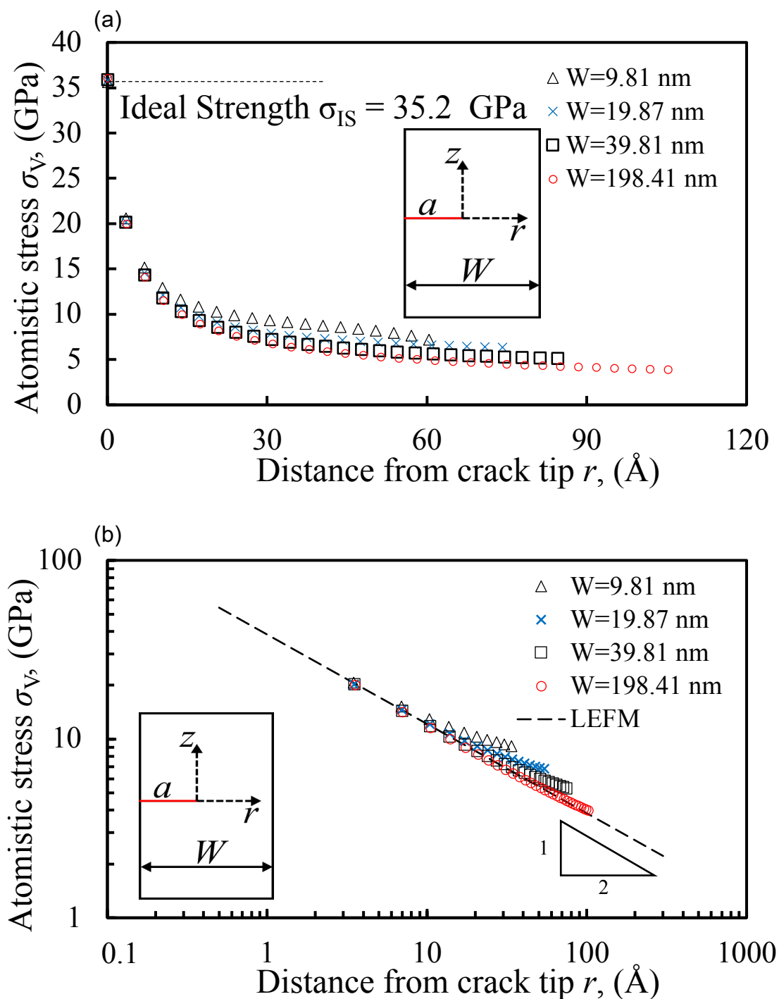
Figure 3. Crack-tip region stress fields from molecular statistics analyses based on virial theorem in (a) linear and (b) log-log scale; \sigma_v is along the z direction, perpendicular to the crack plane.
