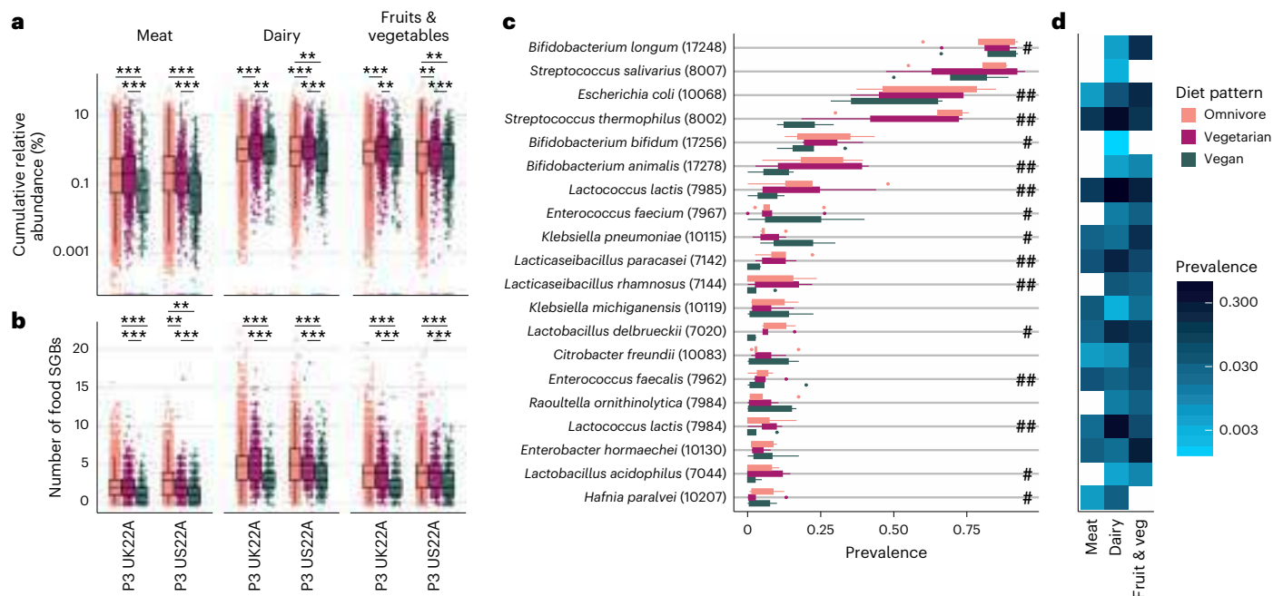
Fig. 5 | Contribution of food microbes to the gut microbiome across diet patterns. a , Cumulative relative abundance (log 10 ) and b , number of food SGBs (either meat, dairy, or fruits and vegetable-derived SGBs) within each individual's gut microbiome, coloured by diet pattern (omnivores: n_{P3UK22A} = 11,533 , n_{P3US22A} = 7,228 ; vegetarians: n_{P3UK22A} = 623 , n_{P3US22A} = 330 ; vegans: n_{P3UK22A} = 197 , n_{P3US22A} = 373 ) and grouped by cohort (either P3 UK22A or P3 US22A; for all cohorts, see Extended Data Fig. 2). Asterisks denote significance level of BH-corrected Dunn's tests; ** P \leq 0.01 , *** P \leq 0.001 (Supplementary Tables 18 and 19). Boxplot parameters the same as in Fig. 1b. c , Prevalence of the 20 most
