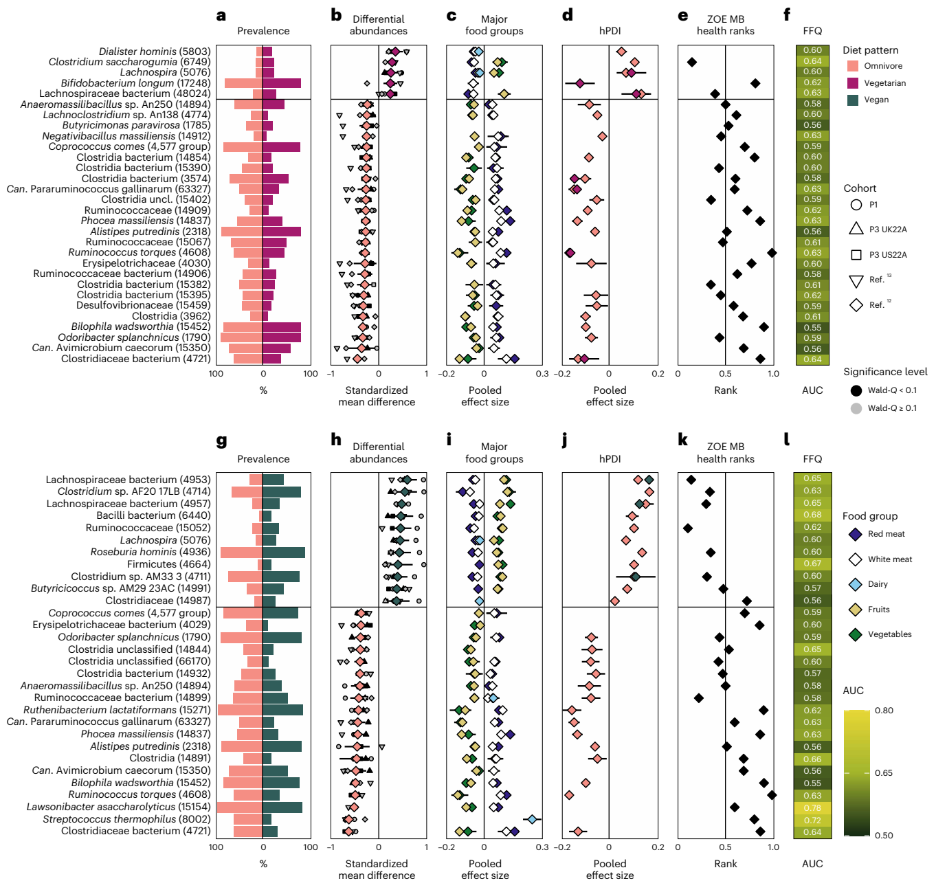
Fig. 3 | Gut microbial signatures of an omnivore vs vegetarian and vegan diets.
