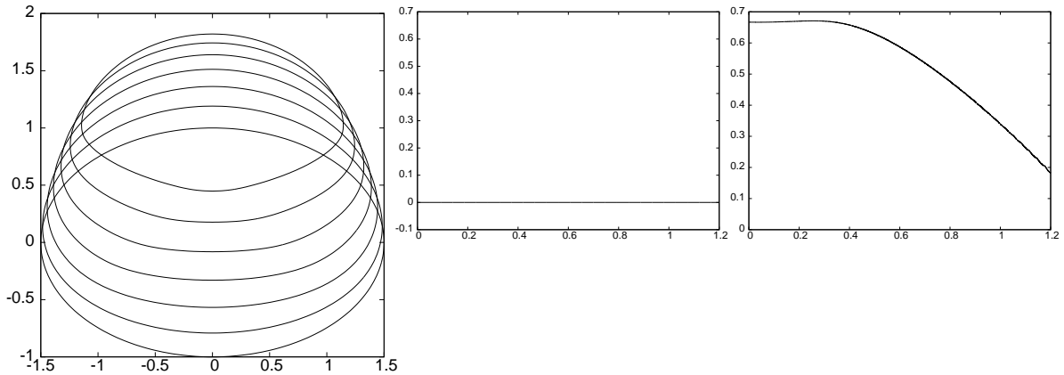
Figure 9: Hyperbolic curvature flow, with \mathcal{V}_0(\rho) = \sin(2\pi\rho) , starting from an ellipse parameterized by x_0(\rho) = (\frac{3}{2} \cos(2\pi\rho), \sin(2\pi\rho))^T . On the left we show \Gamma^m at times t = 0, 0.2, \dots, T = 1.2 . We also show the evolutions of \|D_t x^{m+1} \cdot \theta^m\|_{0,h} (middle) and 1/K_\infty^m (right) over time.
