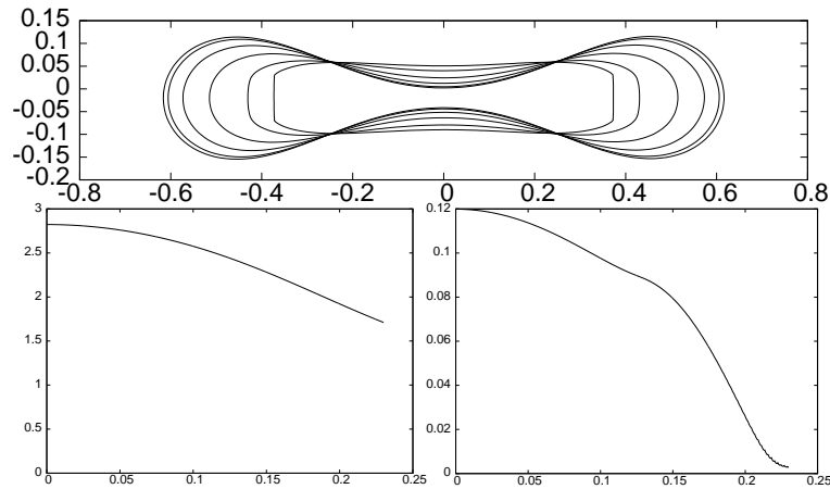
Figure 6: Hyperbolic curvature flow, with V_0 = 0 , starting from a smooth dumbbell. On top we show \Gamma^m at times t = 0, 0.05, \dots, 0.2, T = 0.23 . Below we show the evolutions of |\Gamma^m| (left) and 1/K_\infty^m (right) over time.
