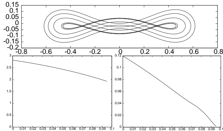
Figure 8: Hyperbolic curvature flow, with V_0 = -1 , starting from a smooth dumbbell. On top we show \Gamma^m at times t = 0, 0.03, \dots, 0.09, T = 0.095 . Below we show the evolutions of |\Gamma^m| (left) and 1/K_\infty^m (right) over time.
