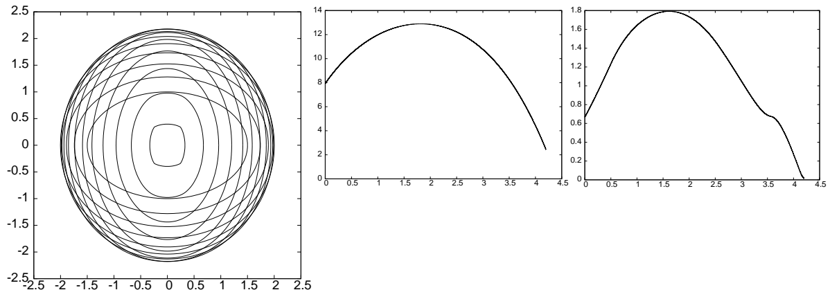
Figure 3: Hyperbolic curvature flow, with V_0 = 1 , starting from an ellipse. On the left we show \Gamma^m at times t = 0, 0.3, \dots, T = 4.2 . We also show the evolutions of |\Gamma^m| (middle) and 1/K_\infty^m (right) over time.
