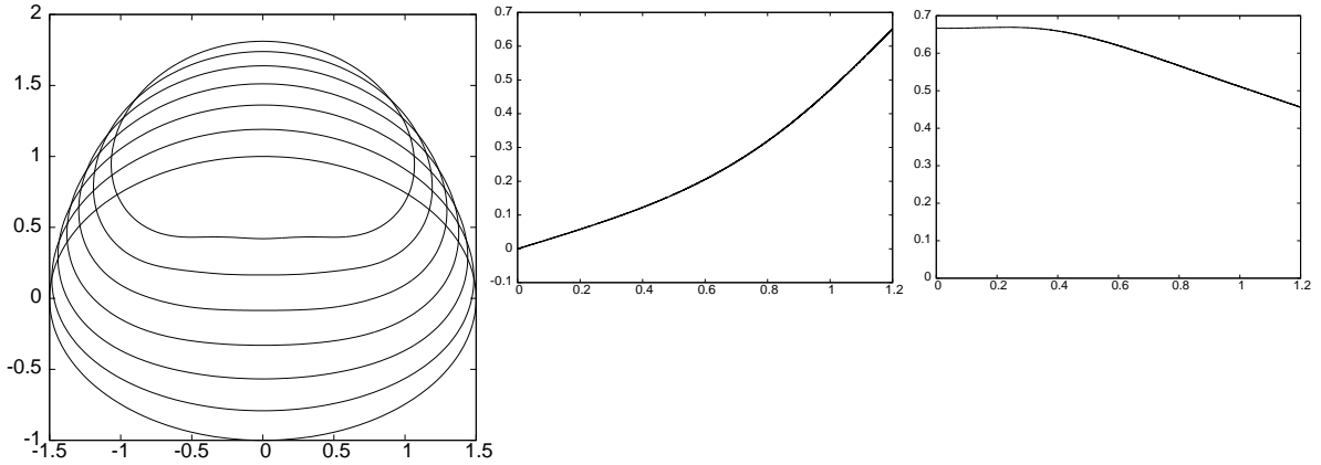
Figure 10: The flow (1.5) with (1.4b) for \mathcal{V}_0(\rho) = \sin(2\pi\rho) , starting from an ellipse parameterized by x_0(\rho) = (\frac{3}{2} \cos(2\pi\rho), \sin(2\pi\rho))^T . On the left we show \Gamma^m at times t = 0, 0.2, \dots, T = 1.2 . We also show the evolutions of \|D_t x^{m+1} \cdot \theta^m\|_{0,h} (middle) and 1/K_\infty^m (right) over time.
