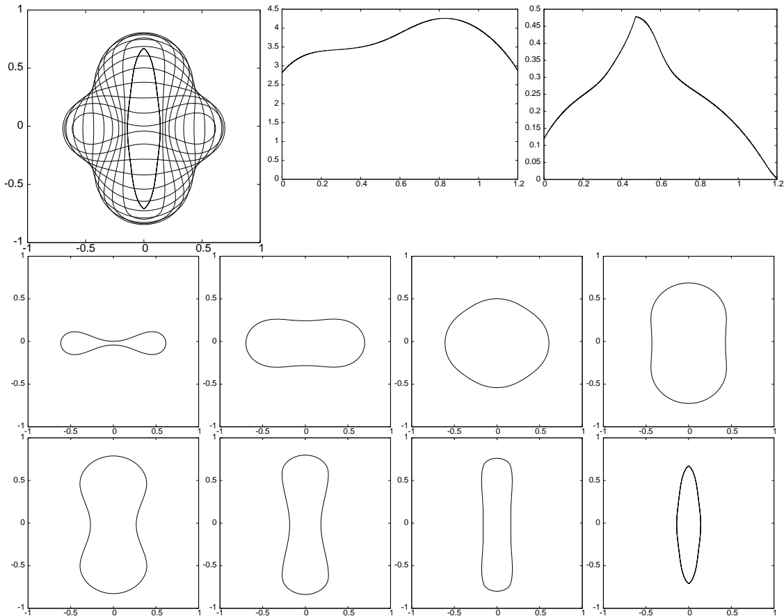
Figure 7: Hyperbolic curvature flow, with V_0 = 1 , starting from a smooth dumbbell. On top we show \Gamma^m at times t = 0, 0.1, \dots, T = 1.2 (left), as well as evolutions of |\Gamma^m| (middle) and 1/K_\infty^m (right) over time. Below we visualize \Gamma^m separately at times t = 0, 0.2, 0.4, 0.6 and 0.8, 1, 1.1, 1.2 .
