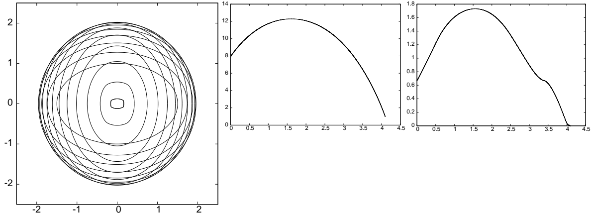
Figure 5: Damped hyperbolic curvature flow, with \beta = 0.1 and V_0 = 1 , starting from an ellipse. On the left we show \Gamma^m at times t = 0, 0.3, \dots, 3.9, T = 4.1 . We also show the evolutions of |\Gamma^m| (middle) and 1/K_\infty^m (right) over time.
