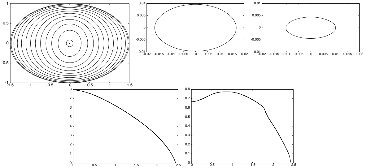
Figure 4: Damped hyperbolic curvature flow, with \beta = 2 and V_0 = 0 , starting from an ellipse. On the top we show \Gamma^m at times t = 0, 0.2, \dots, 2.4, T = 2.4423 , as well as \Gamma^m separately at times t = 2.44 and t = T . Below we show the evolutions of |\Gamma^m| (left) and 1/K_\infty^m (right) over time.
