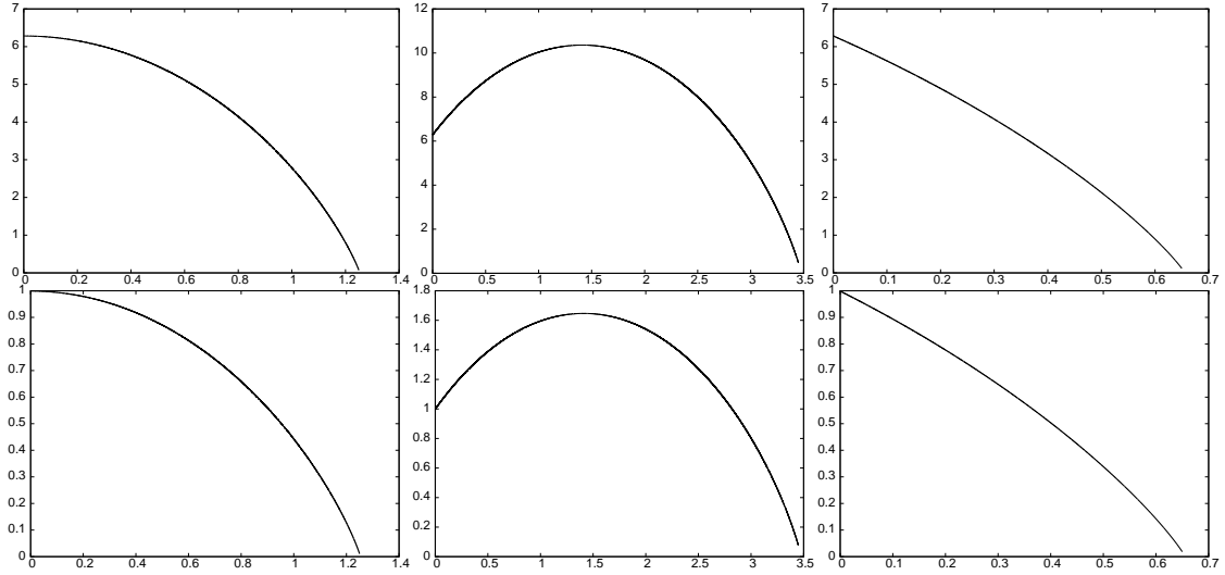
Figure 1: Hyperbolic curvature flow starting from a unit circle. Above we show the evolution of |\Gamma^m| over time for V_0 = 0 , V_0 = 1 and V_0 = -1 (from left to right). The final times for these computations are T = 1.25 , T = 3.45 and T = 0.65 , respectively. Below we show the corresponding evolutions of 1/K_\infty^m over time.
