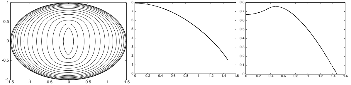
Figure 2: Hyperbolic curvature flow, with V_0 = 0 , starting from an ellipse. On the left we show \Gamma^m at times t = 0, 0.1, \dots, 1.4, T = 1.47 . We also show the evolutions of |\Gamma^m| (middle) and 1/K_\infty^m (right) over time.
