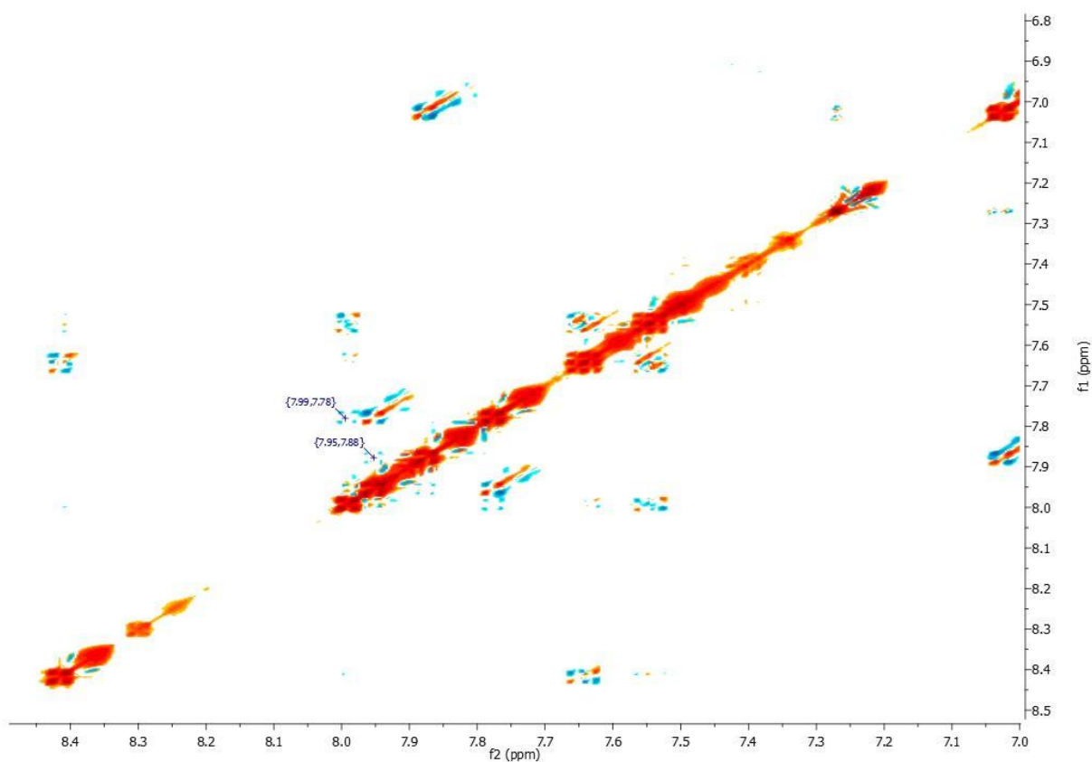
Figure S6: ^1\text{H}, ^1\text{H} spectrum by 2D NOESY experiment (acquired with 0.5 s delay) of the title compound in \text{CDCl}_3 (400 MHz).
