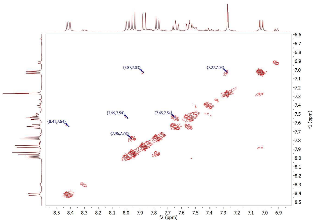
Figure S3: ^1\text{H} , ^1\text{H} correlation spectrum by COSY experiment of the title compound in \text{CDCl}_3 (400 MHz).
