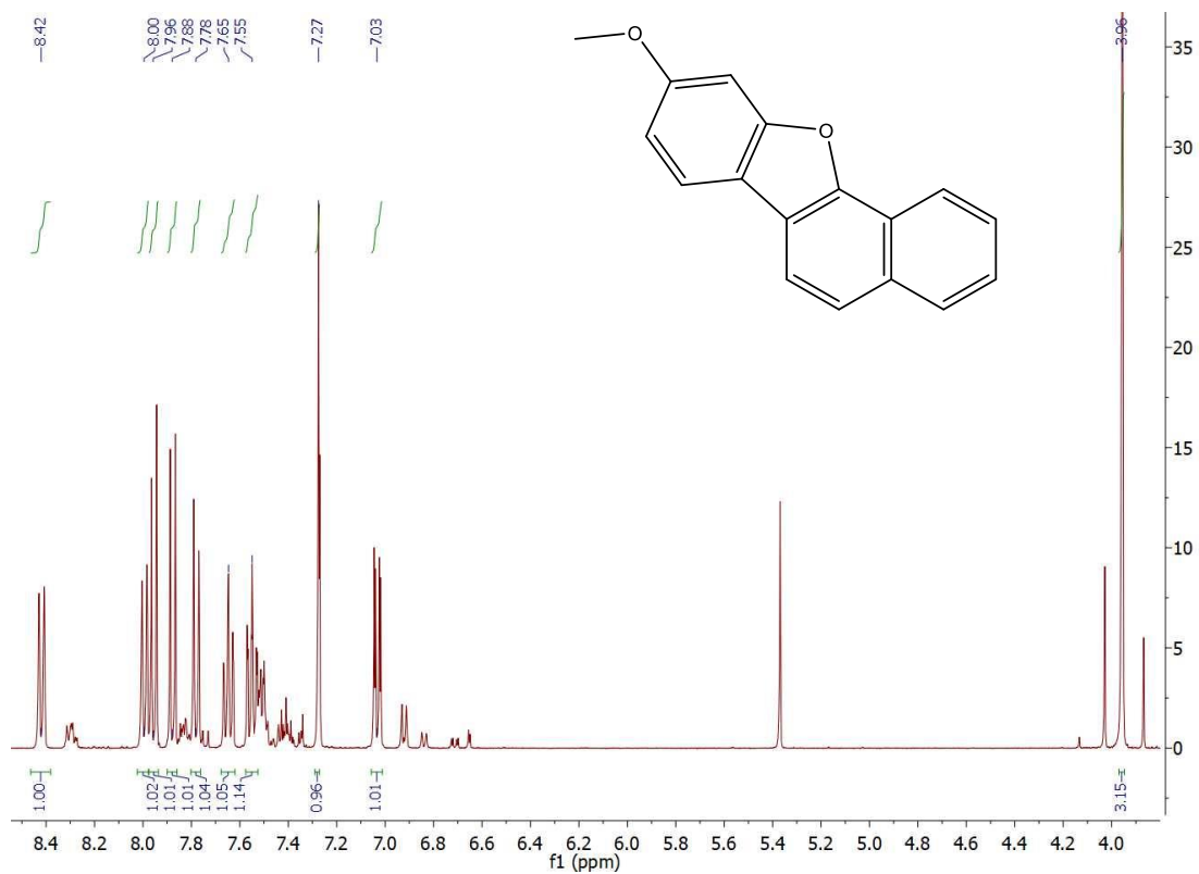
Figure S1: 1 H-NMR spectrum of title compound in CDCl 3 (400 MHz).
