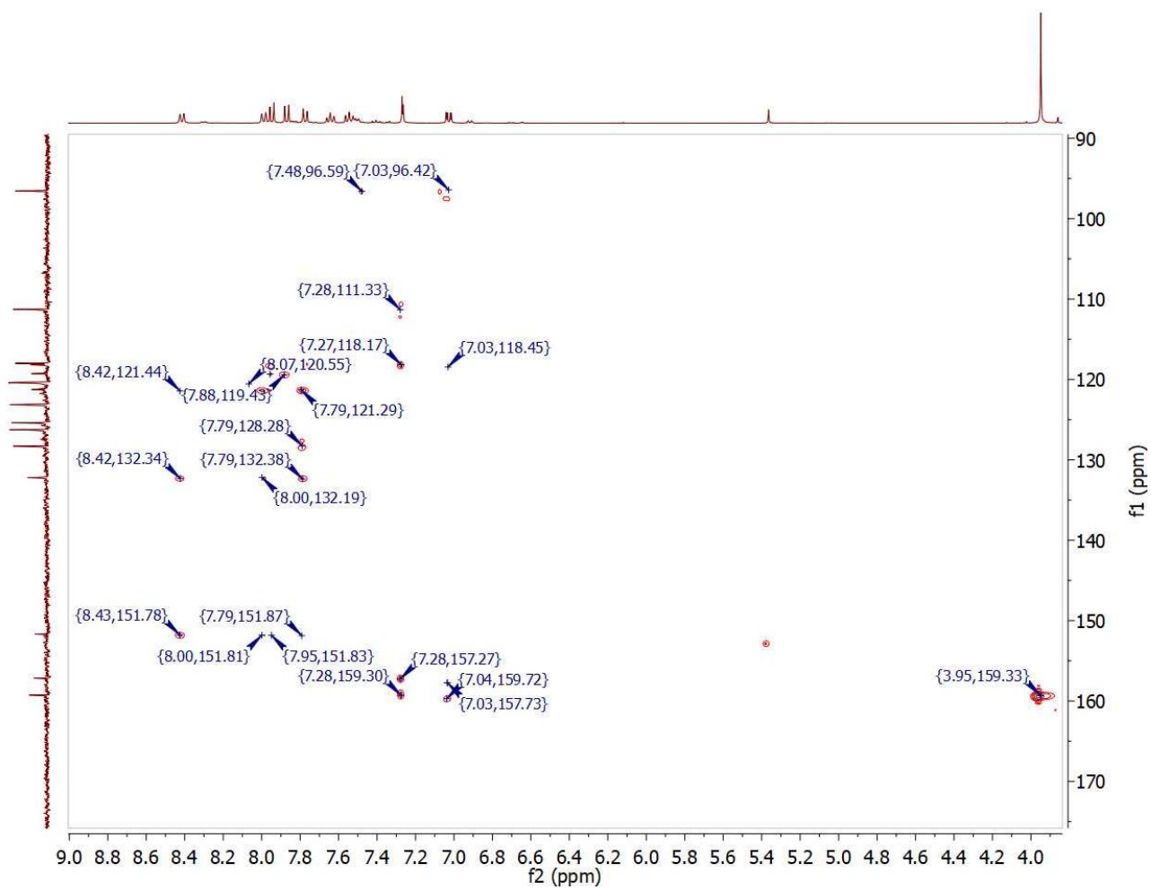
Figure S5: ^1\text{H} , ^{13}\text{C} long range hetero-correlation spectrum by HMBC experiment of the title compound in \text{CDCl}_3 (400 MHz).
