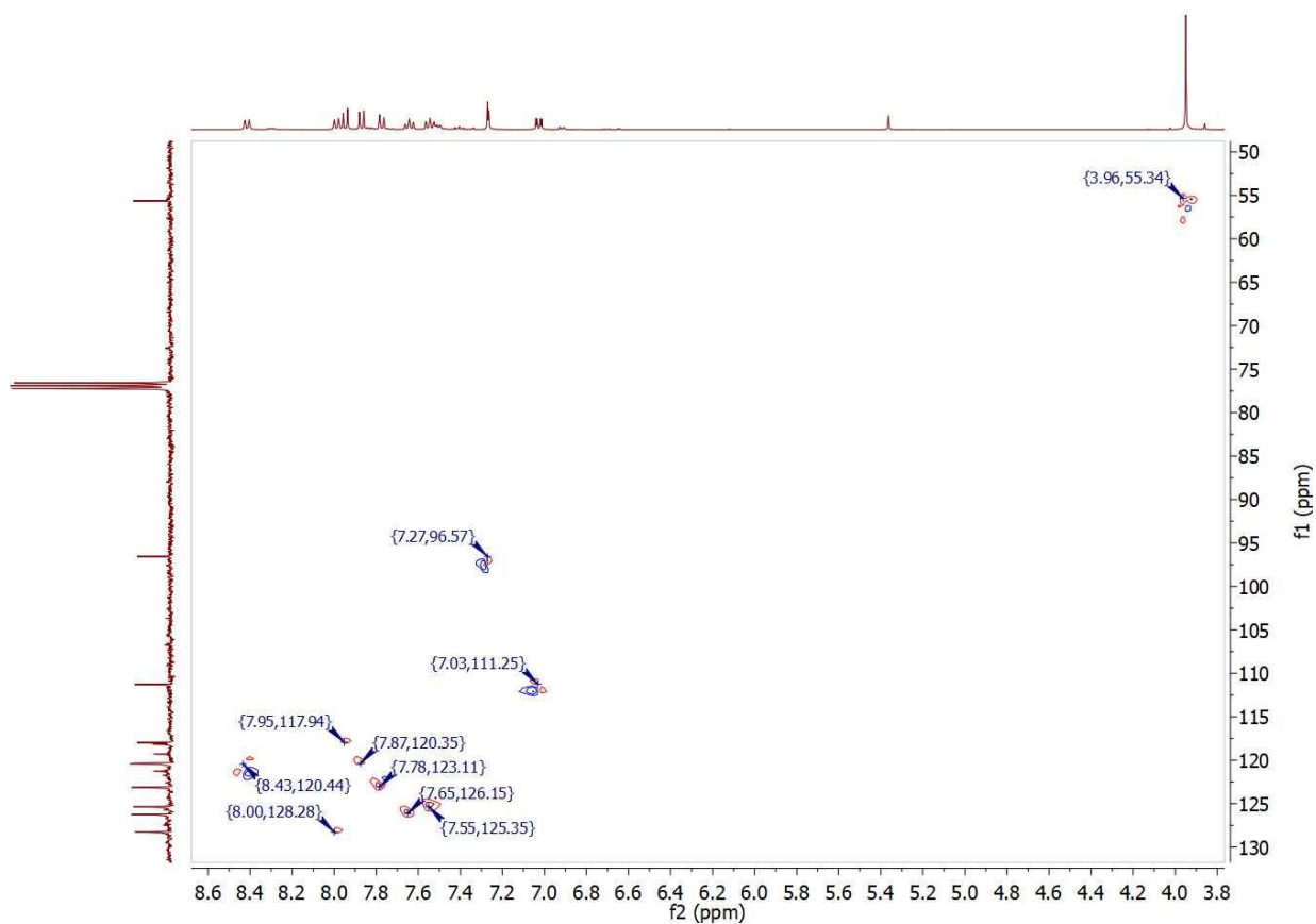
Figure S4: ^1\text{H} , ^{13}\text{C} hetero-correlation spectrum by HSQC experiment of the title compound in \text{CDCl}_3 (400 MHz).
