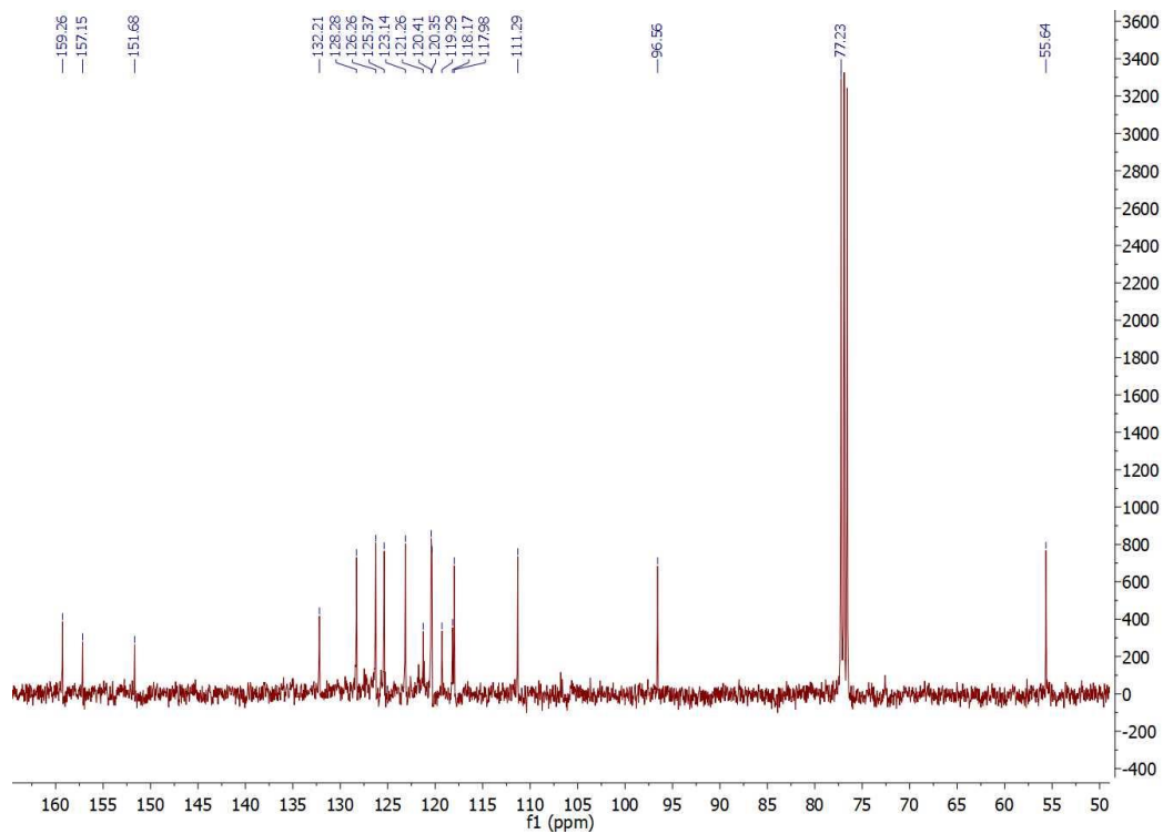
Figure S2: 13 C-NMR spectrum of title compound in CDCl 3 (100 MHz).
