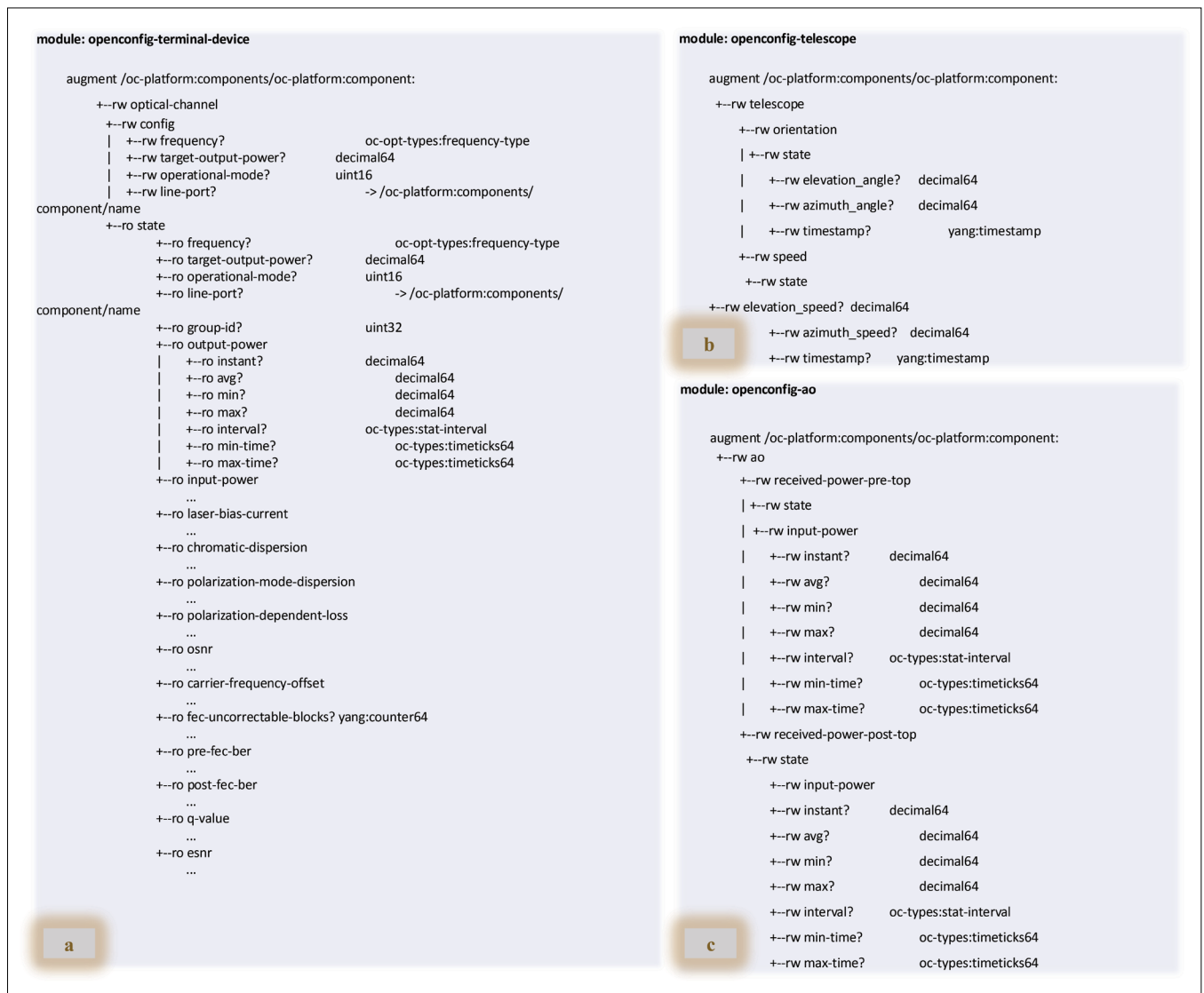
FIGURE 5. a) OpenConfig YANG model; augmentations b) for the telescope, and c) for Adaptive Optics (AO).
