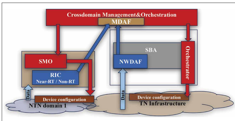
FIGURE 4. Functional architecture of integrated network control system.
