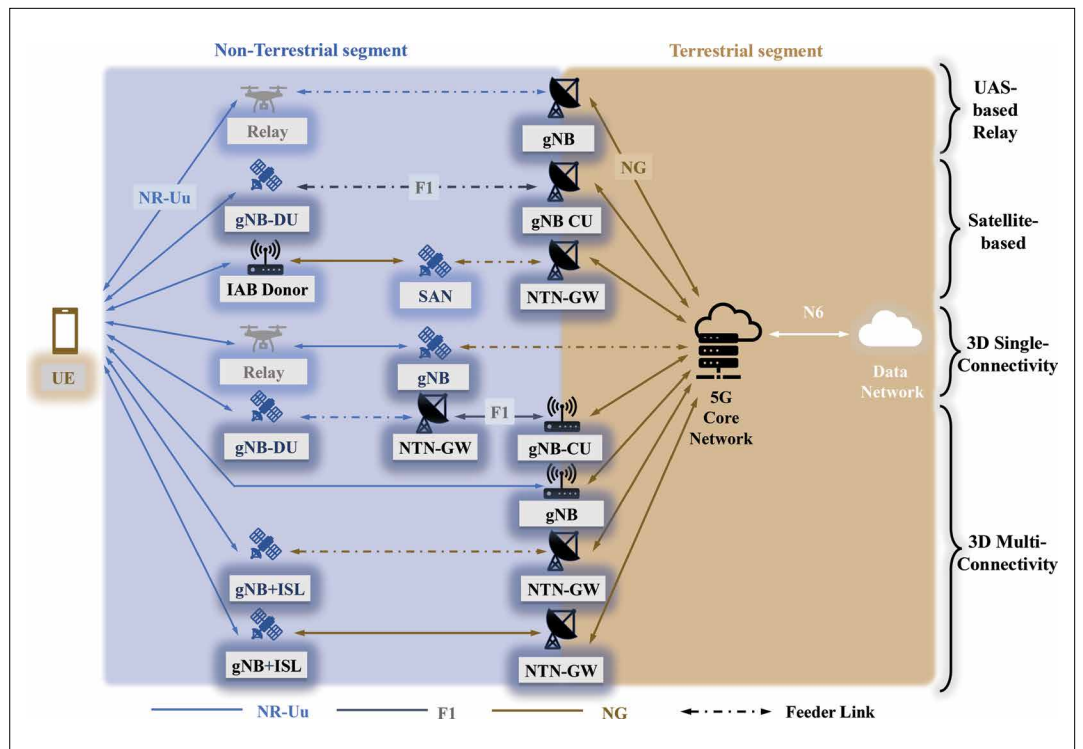
FIGURE 2. Main integrated T/NTN architectures with components and interfaces: UAS-based Relay Network, Satellite-based Architecture, 3D Single-Connectivity Architecture, 3D Multi-Connectivity Architecture.
