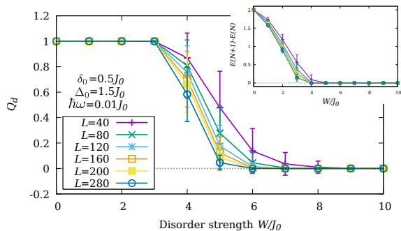
FIG. 1. Disorder average of the diagonal pumped charge plotted against disorder strength. The transition between the quantized charge regime and the trivial one Q_d = 0 is clearly linked to the closing of the minimum energy gap due to the disorder, shown in the inset.
