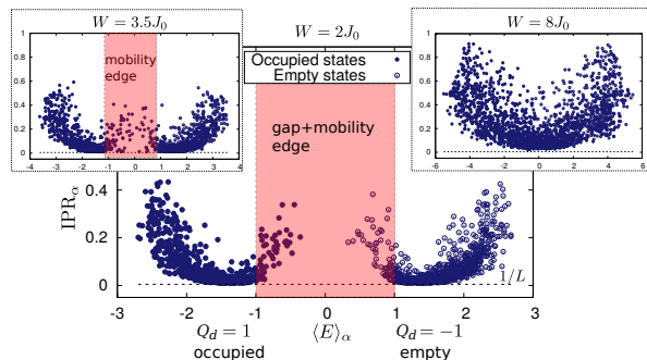
FIG. 3. \text{IPR}_\alpha vs the time-averaged energy of the corresponding Floquet state \langle E \rangle_\alpha . The dashed lines indicate the value 1/L associated to extended states; the data refer to several realizations of a chain with 200 sites and disorder strength W = 2J_0 . In the insets the same data are shown for larger disorder, when delocalized states are separated only by a mobility edge ( W = 3.5J_0 ) and when there is a single band of localized Floquet states ( W = 8J_0 ). Q_d = \pm 1 is the charge transported when a single band, the lower or the higher one, is completely filled.
