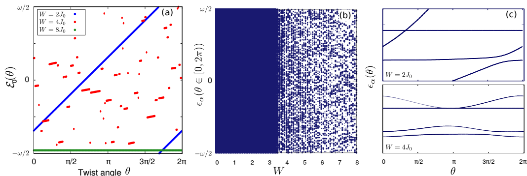
FIG. 4. (a) Quasienergy \mathcal{E}_0(\theta) of the many-body Floquet state with lowest energy. The winding is well defined only for W = 2J_0 and W = 8J_0 , when |\Psi_0\rangle has a non vanishing projection on a single MB Floquet state. (b): SP quasienergy spectrum for all possible angles \theta as a function of the disorder. (c): typical behaviors of SP \epsilon_\alpha(\theta) . When W < W_c most of the states are extended and sensitive to the boundary condition (upper panel), while for W > W_c many quasi-energies do not contribute to the winding, being periodic in \theta (lower panel). All data correspond to the same choice of the random variables \{\zeta_j\} for L = 80 sites. The size of the dots is proportional to n_\alpha(\theta) .
