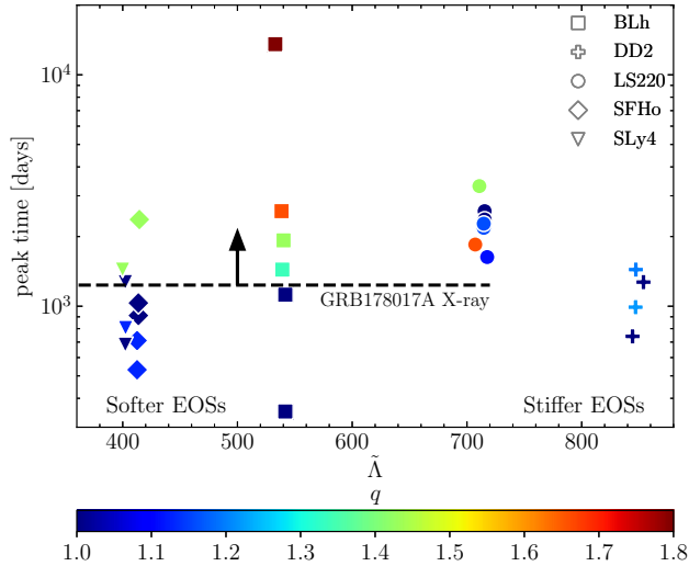
Figure 5. Peak time, t_p , for LCs for all considered NR simulations. Dashed black line corresponds to the last observation of GRB170817A afterglow, where the rising flux implies that it is a lower limit on the kilonova afterglow. The microphysical parameters and ISM density for all models are fixed and given in Table 2. The plot shows that in general the t_p increases with mass ratio and with softness of the EOSs, except for the softest, DD2 EOSs.
