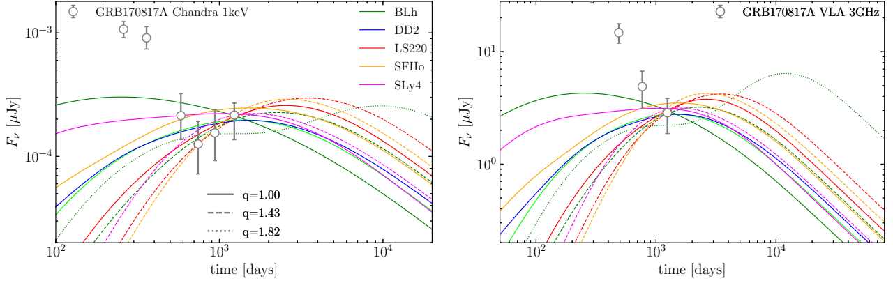
Figure 4. Representative kilonova afterglow LCs for NR models, in X-ray ( left-hand panel ) and in radio ( right-hand panel ), where the grey circles are the observational data from Hajela et al. (2021) and Balasubramanian et al. (2021). The synthetic LCs are computed with varying microphysical parameters and ISM density within the range of credibility to achieve a better fit to observational data (see Table 2 for details). The plots show that, within allowed parameter ranges, the LCs from all models are in agreement with observations. Models with moderately stiff EOSs and q < 1 < 1.8 are tentatively preferred, as their flux is rising at t \geq 10^3 d, in agreement with observations.
