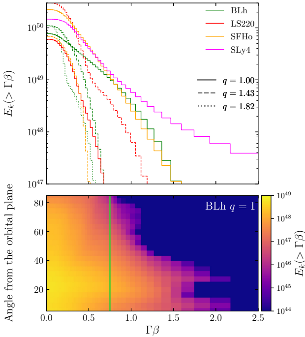
Figure 3. Cumulative kinetic energy distribution for a selected set of models ( top panel ) and its angular distribution for a BLh q = 1.00 model ( bottom panel ). The vertical light green line marks the v_{ej} = 0.6 . The top panel shows that equal mass models have a more extended high energy tail, while the bottom panel shows that the angular distribution of the ejecta is not uniform.
