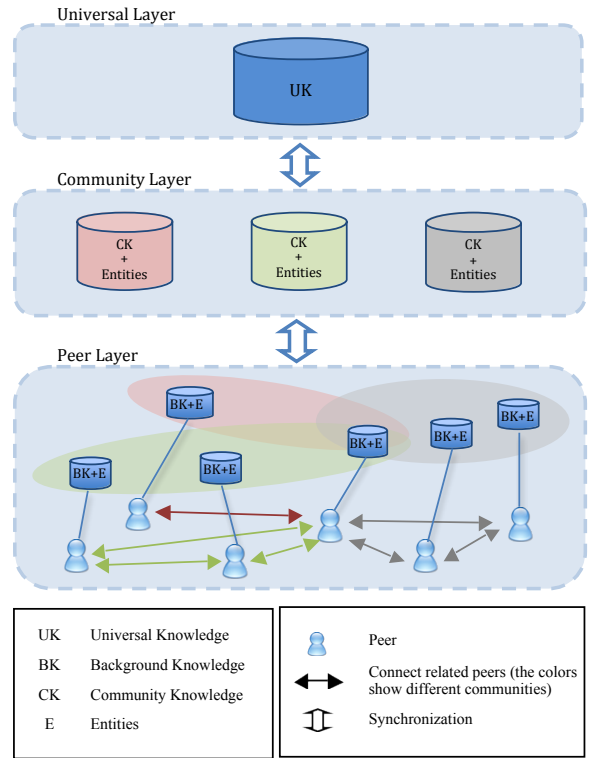
Figure 1: Logical architecture.
