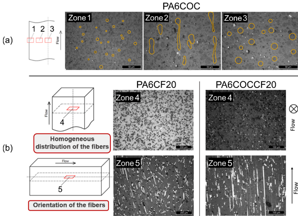
Fig. 2. Light optical micrographs of the prepared samples. (a) Schematic representation of the three different locations where the specimens of PA6COC were taken and micrographs of the polished cross-sections of the corresponding zones. (b) Schematic representation of the location where the specimens of PA6CF20 and PA6COCCF20 were taken and micrographs of the polished cross-sections of the corresponding zones. Arrows represent the direction of material flow during injection molding. White dots are caused by light reflection on the CFs.
