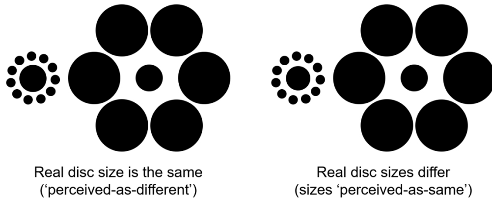
Figure 1. The Ebbinghaus display devised for the current study. Inner black-filled circles are surrounded by an annulus of small or large black-filled circles. Two versions of the display are illustrated, one in the left panel and one in the right, and each display is presented as a ‘dual’ configuration. Left panel: the traditional presentation in which the real sizes of the inner discs are the same but are misperceived as different. This is the critical feature of the display on ‘perceived-as-different’ trials. Right panel: a version in which the real sizes of the inner discs are different, leading to the impression that they are the same size. The difference in size required to achieve this varies from person to person, but it is scaled here to the most common difference in the study (2mm). A pair of discs whose real sizes were different to make them appear to be the same in size is the critical component of the ‘perceived-as-same’ display.
