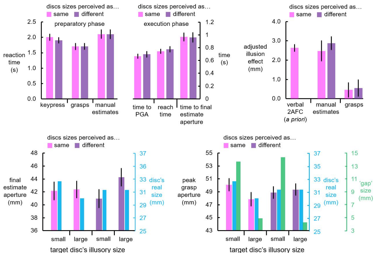
Figure 2. Top left: Preparatory and execution phase temporal dependent measures as a function of task and display type. The grasps were initiated the fastest, and the mean initiation time for the estimates and the mean keypress time for the keypress task were statistically equivalent. With respect to the execution phase, the reach time for the grasps was faster than the final estimate aperture time. Top right: the a priori effect of the Ebbinghaus illusion, using the 'perceived-as-same' display (established in the initial verbal 2AFC task), and the adjusted effects of the Ebbinghaus illusion on the manual estimates (middle) and grasps (right) as a function of display type. The effect of the illusion on the estimates was comparable to the a priori effect, whereas the effect of the display on the grasps was null. Bottom panels: Peak grasp aperture for the grasps (left) and final estimate aperture for the manual estimates (right) as functions of the direction of the effect of the illusion ("small" – the inducer decreases the perceived size of the target; "large" – the inducer increases the perceived size of the disc) and the display type (i.e., the perceived-as-
