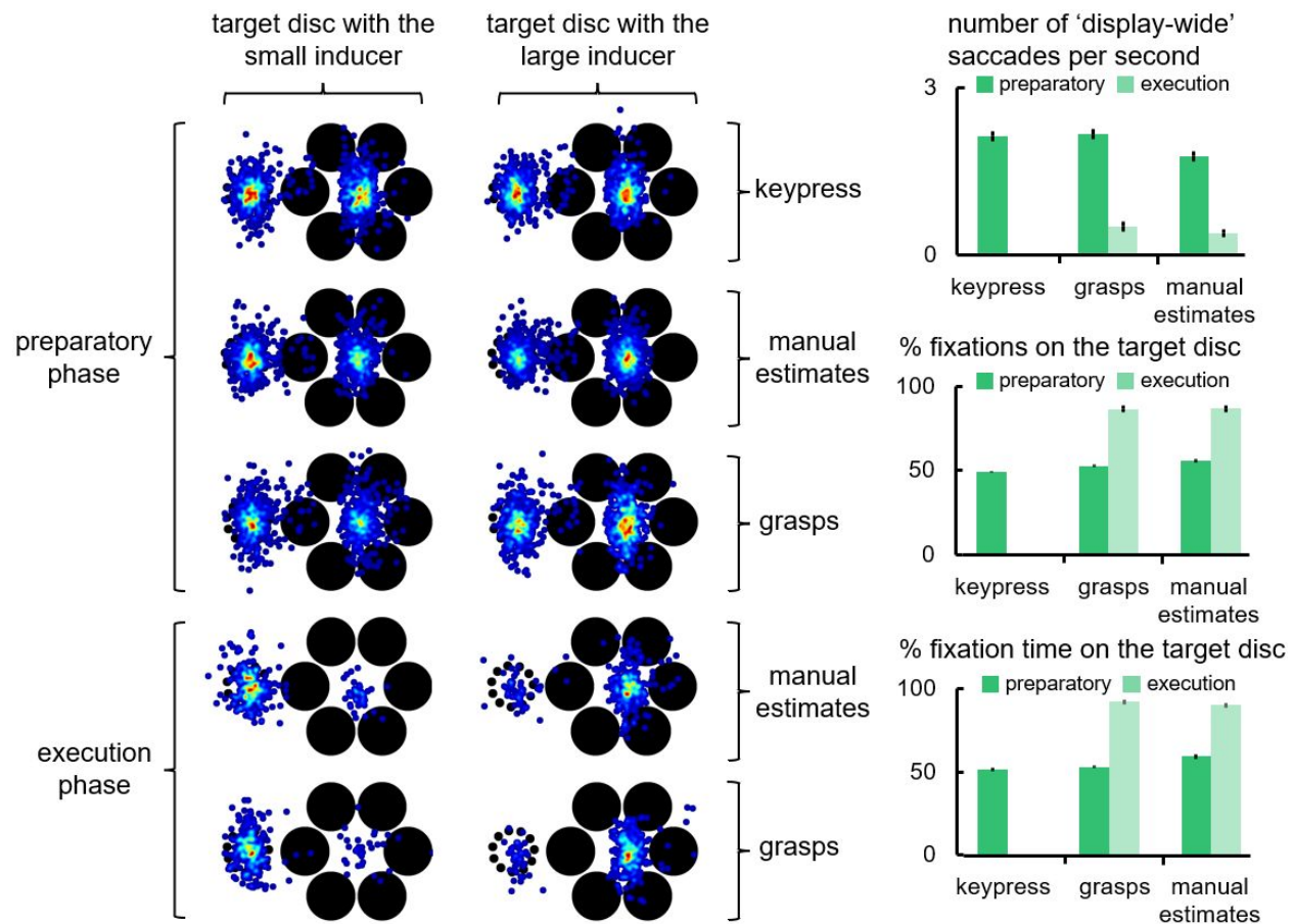
Figure 3. The spatial distribution of fixations and the fixation measures as functions of task and the response phase (i.e., the preparatory and execution phases). Left: gaze maps show the spatial distribution of fixations parsed into trials in which the target disc was surrounded by the small or large inducer. Display orientation is collapsed such that fixations on those trials with the opposite board orientation to the one depicted were flipped across the central vertical axis of the full set of fixations. Top right: The number of 'display-wide' saccades (gaze shifts between disc positions two or more locations apart from one another) per second. Middle right: The percentage of total fixations that were directed at the target disc. Bottom right: The percentage of total fixation time that was directed at the target disc and inducer (right). During the preparatory phase, participants made more saccades between the discs, fixated on the target disc less, and spent less fixation time on the target, relative to the execution phase. Moreover, none of the fixation measures during the preparatory phase differentiate the keypress and manual estimation tasks from the grasping task. During the execution phase, the fixation measures fail to differentiate the grasps and manual estimates. Error bars are SEMs.
