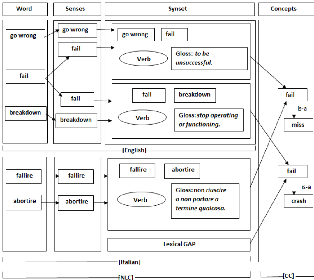
Figure-1: The relation between the English word “fail”, its word senses, synstes and concepts together with the Italian word “fallire”, its word senses, synsets and concepts. Concepts are language independent but in this figure instead of providing the concept ID, we show concept labels in English.
