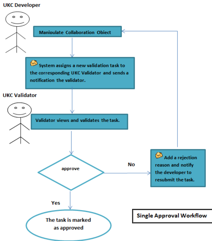
Figure 3. Single Approval Workflow
