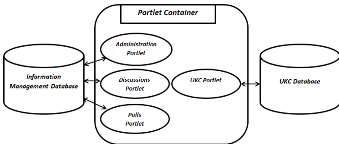
Figure-5 UKC Collaborative Platform Overall Architecture
