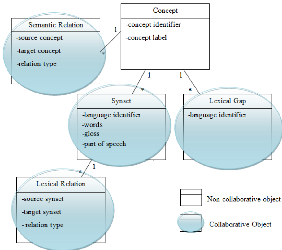
Figure 2. Collaborative and non-collaborative objects in UKC
