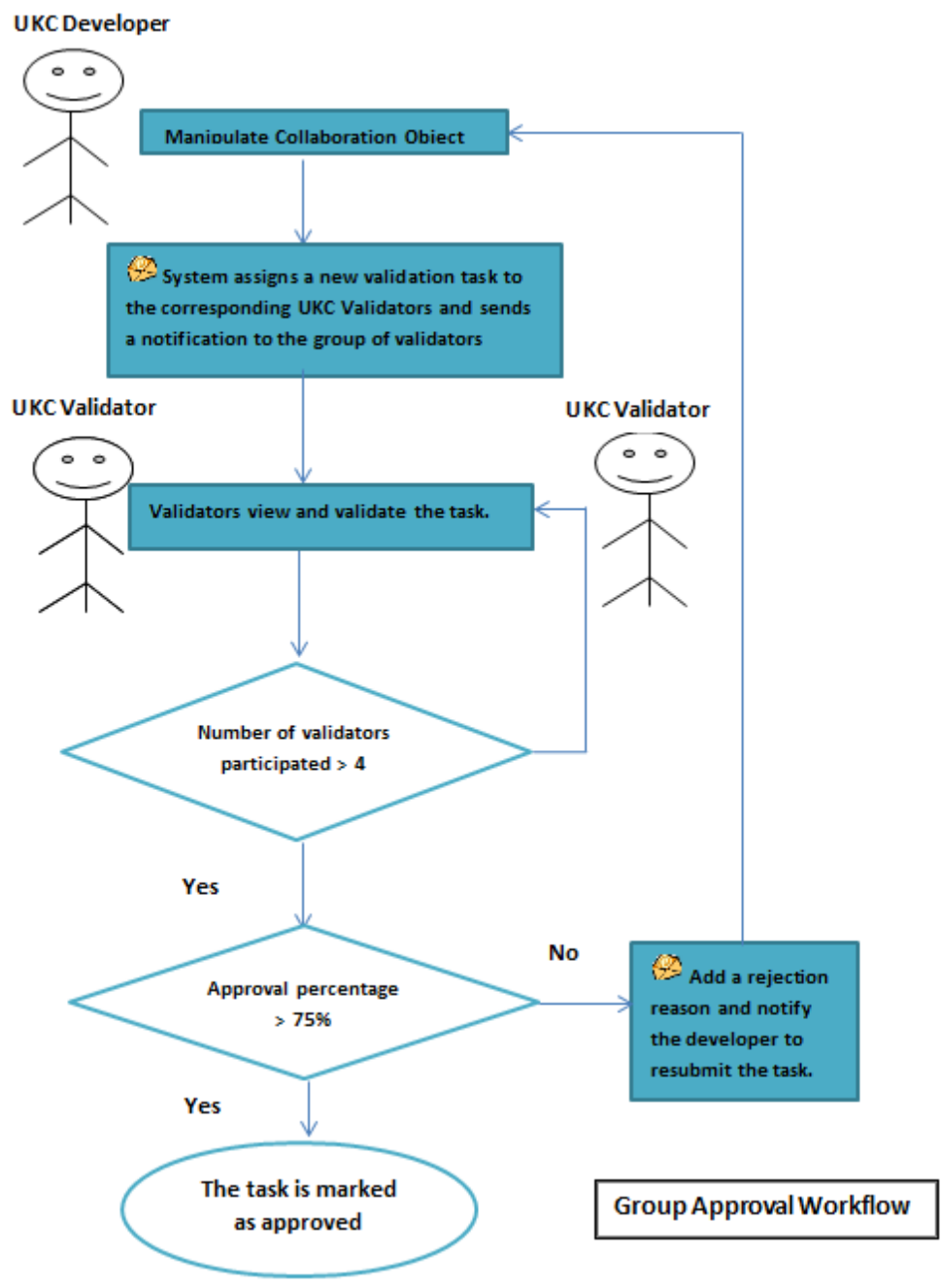
Figure 4. Group Approval Workflow
