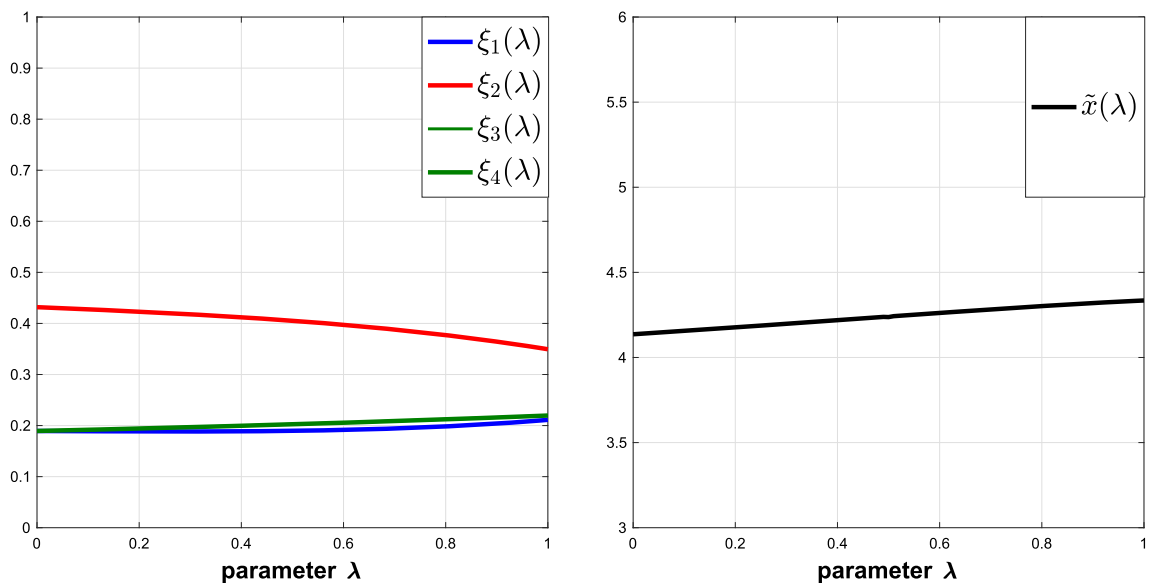
Fig. 14 The change of \xi_1(\lambda) , \xi_2(\lambda) , \xi_3(\lambda) , \xi_4(\lambda) and the change of the consensual opinion \tilde{x}(\lambda) as the parameter \lambda increases
