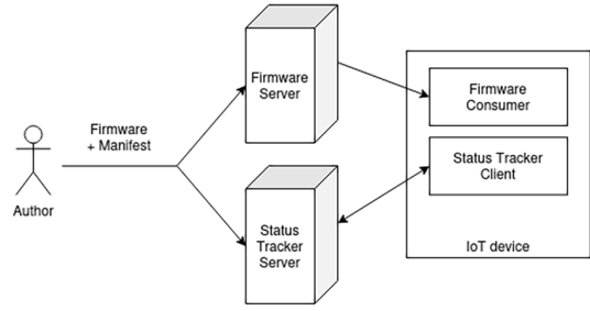
Fig. 1. The SUI secure update architecture.
