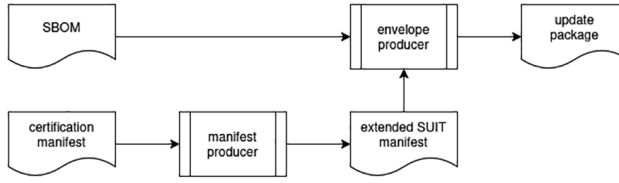
Fig. 4. Workflow for the generation of the Update Package.
