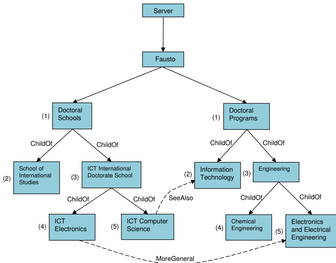
Figure E.1: An example of a classification rooted at Server.
