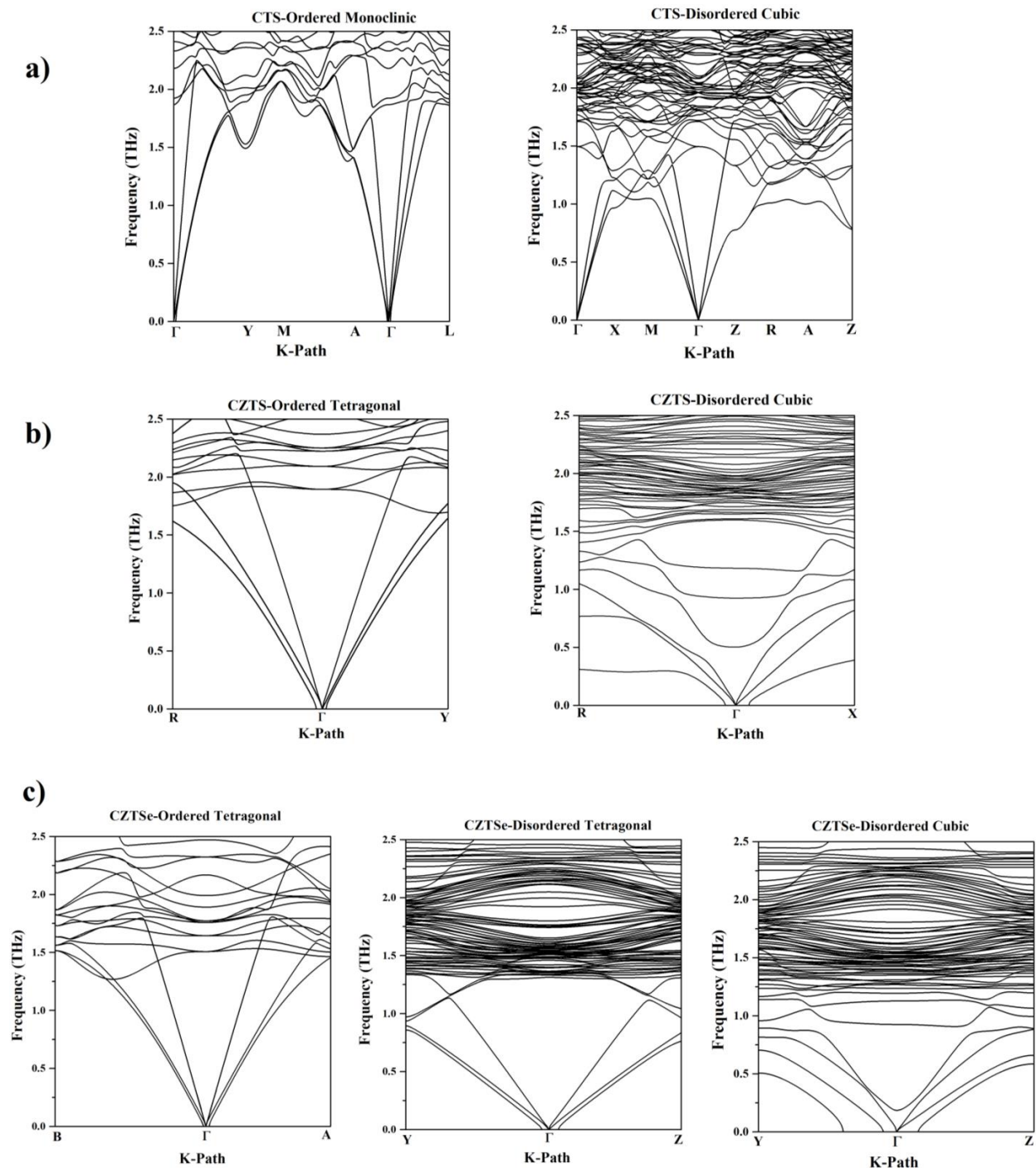
Figure 8. Phonon dispersion curve for CTS (a), CZTS (b), and CZTSe (c) polymorphs. The effect of structural disorder on the phonon dispersion curve manifests itself in the form of a gentle slope of the acoustic branches and the low-lying optical modes.
