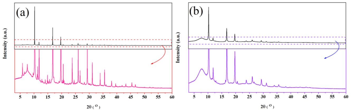
Figure 1. SR-XRD measurements on monoclinic (a), and cubic (b) \text{Cu}_2\text{SnS}_3 polymorphs collected at 350^\circ\text{C} . The zoomed images show the superstructure Bragg peaks ( 2\theta < 10^\circ ) for monoclinic CTS phase representing (110), (11-1), and (021) reflections. These superstructure Bragg peaks are absent for the cubic CTS phase. The broad peak with diffused background at low 2-theta is due to the use of borosilicate glass for the dilution of samples.
