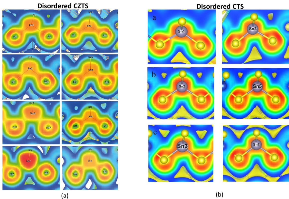
Figure 9. The calculated electron localization function mapped on to the Sn-S bonds in (a) disordered CZTS and (b) disordered CTS. The ELF distribution for certain Sn ions shows a strong bonding inhomogeneity in both systems, with only CZTS showing lone-pair localization in a fraction of ions (for example see Sn7 in the panel in the bottom left corner of the figure). These images are taken from [34,52].
