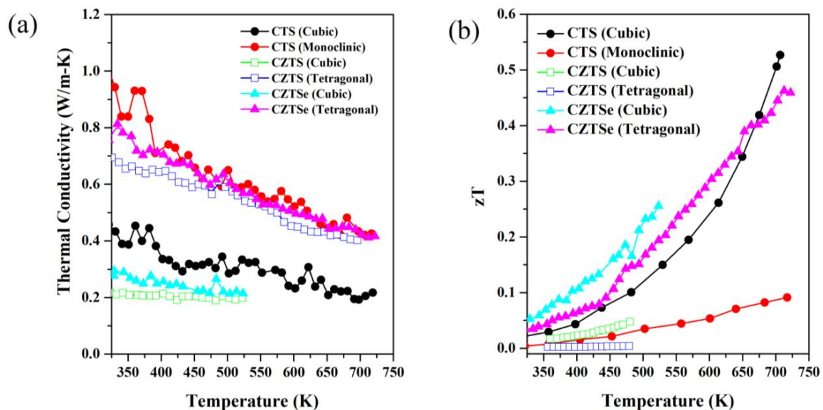
Figure 7. Temperature-dependent thermal conductivity (a) and zT (b) for CTS, CZTS, and CZTSe polymorphs data retrieved from [20,34,51,52].
