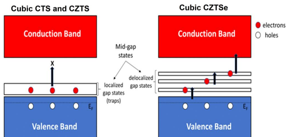
Figure 6. A schematic diagram showing the effect of mid-gap states: In cubic CTS/CZTS, the localized nature of these states acts to unilaterally enhance hole concentration at finite temperature by ‘trapping’ electrons. For cubic CZTSe instead, these states are delocalized within the gap, and therefore do not act as traps.
