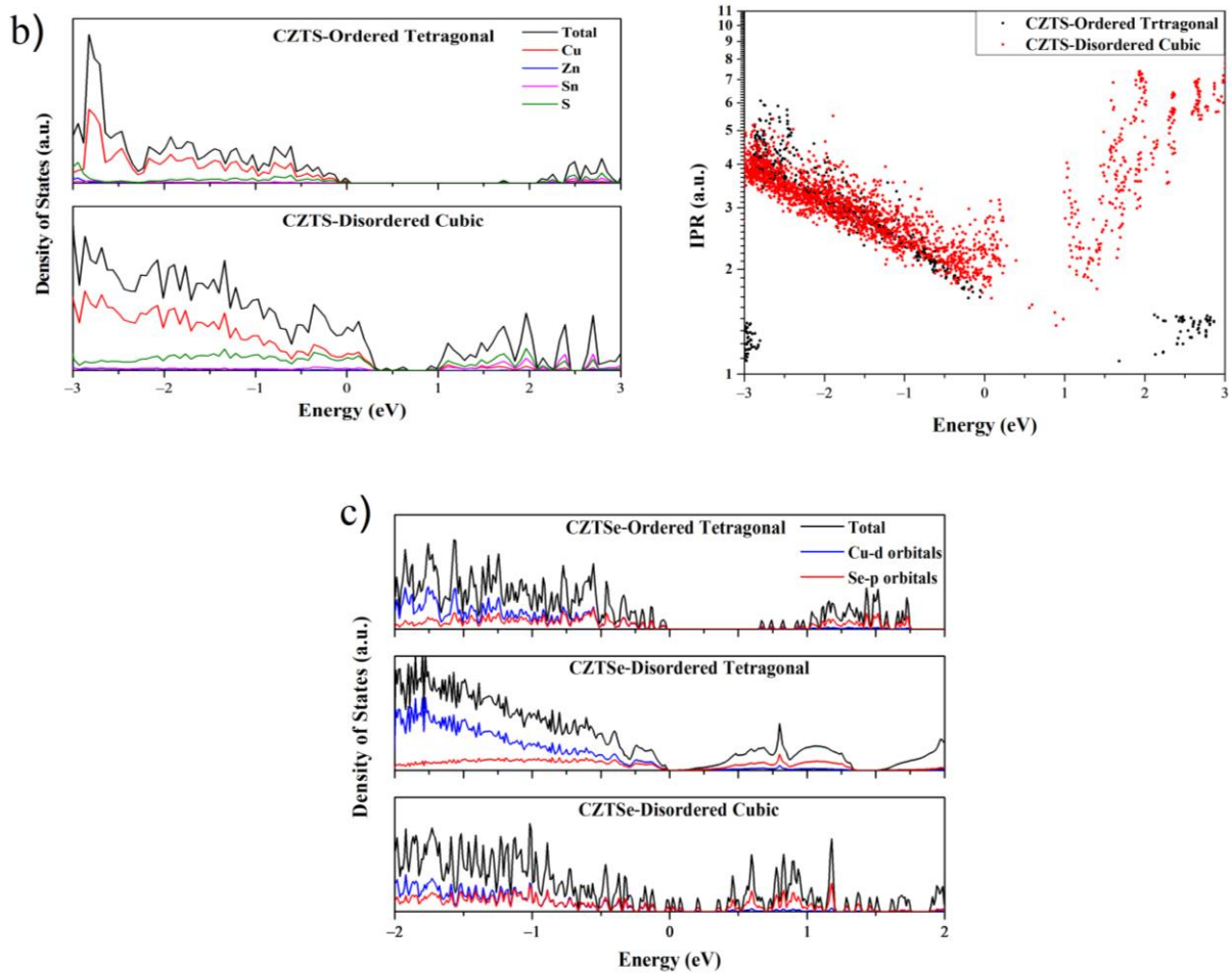
Figure 5. The total and atomic projected electronic density of states for CTS ordered monoclinic, CTS Disordered Cubic 1 (Cu-21, Sn-11, S-32), and CTS Disordered Cubic 2 (Cu-22, Sn-10, S-32) (a), CZTS (b), and CZTSe (c) polymorphs. Here, the Fermi level is set to zero. The IPR for the CTS and CZTS shows localized states near the Fermi level.
