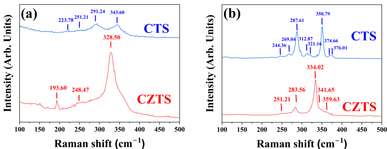
Figure 3. Raman spectra collected with a 488 nm laser on as-milled (a) and thermally treated (b) samples of CTS and CZTS. The samples in (a), in the disordered cubic phase, display significantly broader peaks than the ordered (monoclinic CTS and tetragonal CZTS) phases in (b). This is believed originating from cation disorder itself, likely causing variable coordination environments and inhomogeneous bonds, leading to a spread in vibrational modes.
