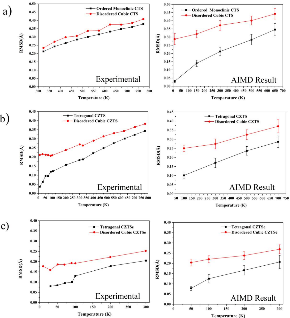
Figure 2. Temperature variation of RMSD calculated from SXRD and AIMD simulation for CTS (a), CZTS (b), and CZTSe (c).
