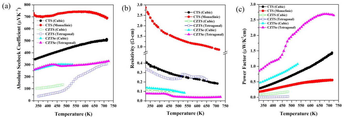
Figure 4. Temperature-dependent Seebeck coefficient (a), electrical resistivity (b), and power factor (c) curves for CTS, CZTS, and CZTSe polymorphs retrieved from [20,34,51,52].
