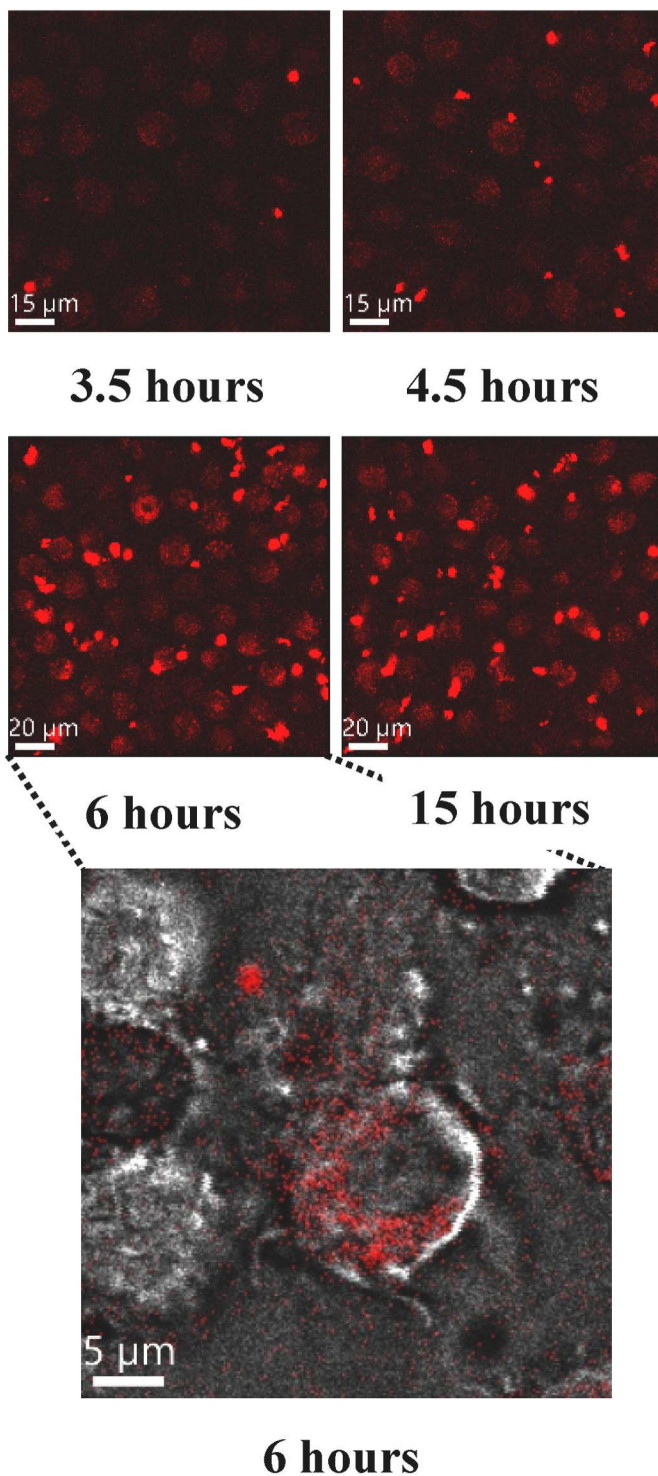
Fig. 5. Overnight frames (3.5, 4.5, 6 and 15 h after the treatment) of live-cell imaging of DCs treated with pSi microparticles loaded with Pam3CSK4-R displayed through the red channel (15 and 20 \mu\text{m} ). A magnification of the 6 h image showing a DC treated with pSi microparticles loaded with Pam3CSK4-R and the signal distribution (5 \mu\text{m} scale) is illustrated in the bottom panel. (For interpretation of the references to colour in this figure legend, the reader is referred to the Web version of this article.)
