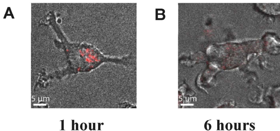
Fig. 7. Live-cell confocal images of DCs treated with (A) soluble Pam3CSK4-R and (B) with pSi microparticles loaded with Pam3CSK4-R (532 nm laser excitation, frames at 1 and 6 h, respectively) (5 \mu m scale).
