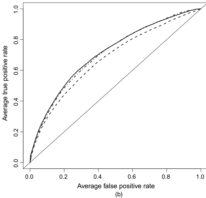
46 Fig. 7. Receiver operating characteristic curves for default prediction models under the inclusion of various 47 sets of variables, calculated on test data and averaged across 50 75%–25% training-test splits (----, 48 + company characteristics; - · - · - ·, + network characteristics; ·····, + characteristics of neighbours; —, + failure of neighbours): (a) Logistic regression; (b) random forests
