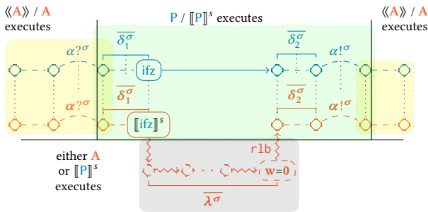
Figure 2: Diagram depicting the proof that \llbracket \cdot \rrbracket^s is RSSC.
