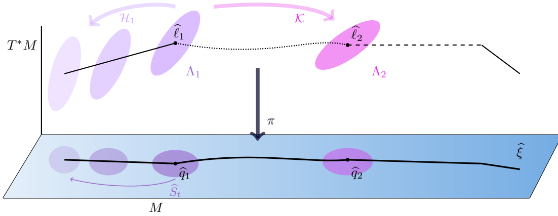
FIGURE 1. Invertibility for t \in [0, \widehat{\tau}_3] : \mathcal{H}_t(\Lambda_1) projects diffeomorphically onto a neighbourhood of \widehat{\xi}(t) for every t \in [0, \widehat{\tau}_3] .
