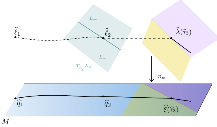
FIGURE 2. Invertibility at t = \hat{\tau}_3 . L_+ (respectively, L_- ) denotes the half space of all \delta \ell_2 \in T_{\hat{\ell}_2} \Lambda_2 such that \langle d\hat{\tau}_3(\hat{\ell}_2), \delta \ell_2 \rangle \geq 0 (respectively, \leq 0 ). In purple, \mathcal{H}_{\hat{\tau}_3} L_+ ; in yellow, \mathcal{H}_{\hat{\tau}_3} L_- . These semi-planes project without intersections on T_{\hat{\xi}(\hat{\tau}_3)} M .
