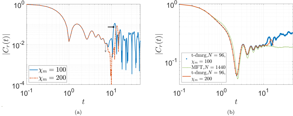
FIG. 23. Non-equilibrium responses calculated with t-DMRG for weakly interacting TFIM with \Delta/J = 0.1 at N = 96 are compared with respect to different maximum bond dimensions, \chi_m = 100 and \chi_m = 200 which is introduced as an approximation in the t-DMRG algorithm to simulate for longer times, see Sec. IV C. The comparison is shown in subfigures (a) at h/J = 1.3 and (b) at h/J = 1 . (a) With increasing bond dimension, a downward moving envelope appears in the t-DMRG result, emphasized by the dotted-gray arrow, agreeing with the qMFT results in the disordered phase. The solid-black arrow points to the effects of finite bond dimension. (b) The qMFT result at N = 1440 is compared with the t-DMRG results. We notice the convergence of the t-DMRG result with greater \chi_m (red-solid) to the qMFT result (green-dotted) for a small time interval that was accessible, before showing the effects of finite bond dimension.
