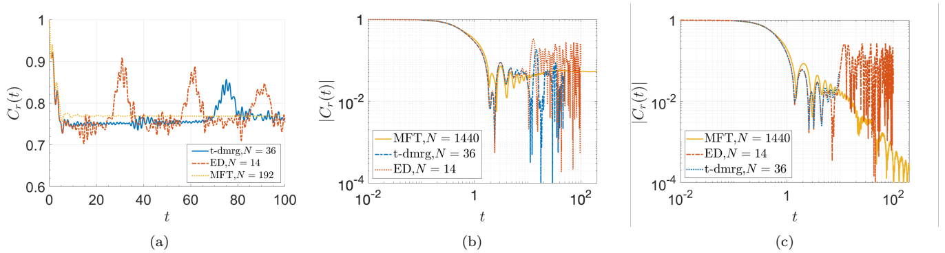
FIG. 22. Benchmarking qMFT analysis. All subfigures compare the results of qMFT, t -DMRG and exact diagonalization (ED) results (see individual legends for system sizes) for C_3(t) . The external fields are (a) h = 0.5 , (b) h = 1.1 and (c) h = 1.2 . In all subfigures, the qMFT nonequilibrium response matches sufficiently well with the nonequilibrium responses of the exact methods, in particular in early times close to QPT and in the disordered phase where exact methods are constrained either by finite-size (ED algorithm) or finite bond dimension and short simulation times ( t -DMRG algorithm).
